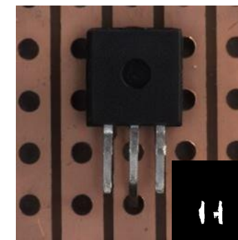
transistor-misplaced
