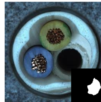
cable-missing cable
