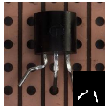
transistor-bent lead
