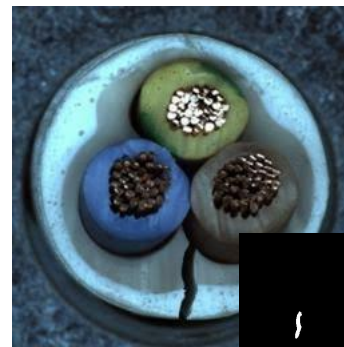
cable-cut outer insulation
