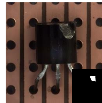
transistor-damaged case
