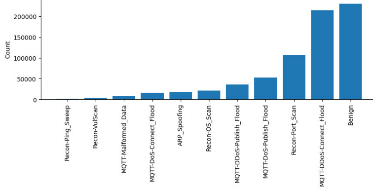
Figure 3: Distribution of multi-class attack data. Source: [25]
