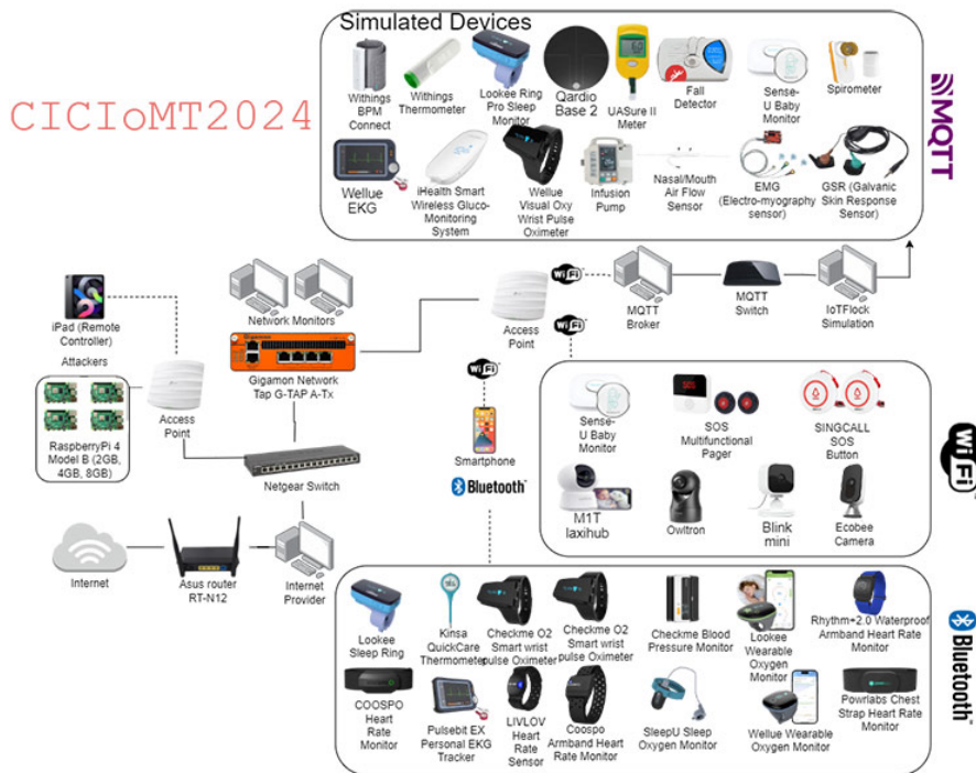
Figure 2: CICIoMT2024 topology. Source: [8]
