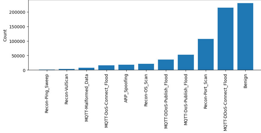
Figure 3: Distribution of multi-class attack data in the CIC2024IoMT dataset. Source: [25]
