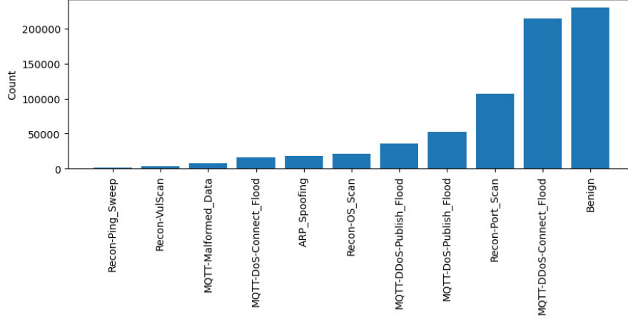
Figure 3: Distribution of multi-class attack data in the CIC2024IoMT dataset. Source: [25]
