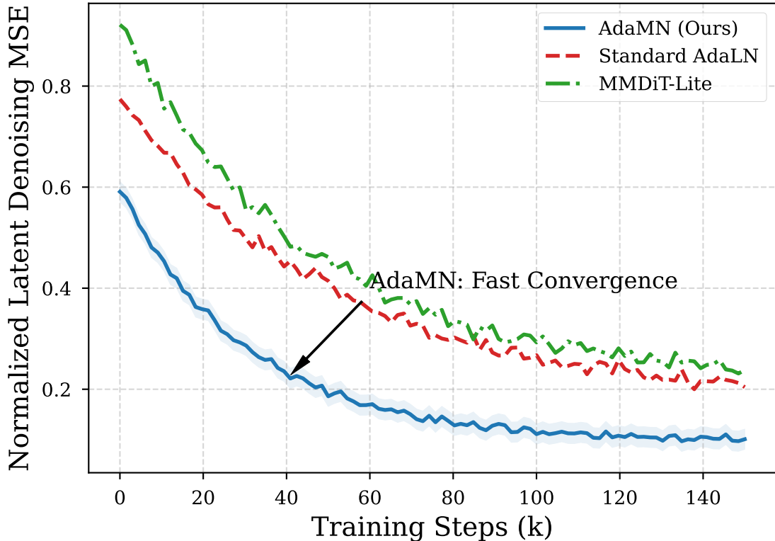
Convergence Efficiency of Modality Alignment
