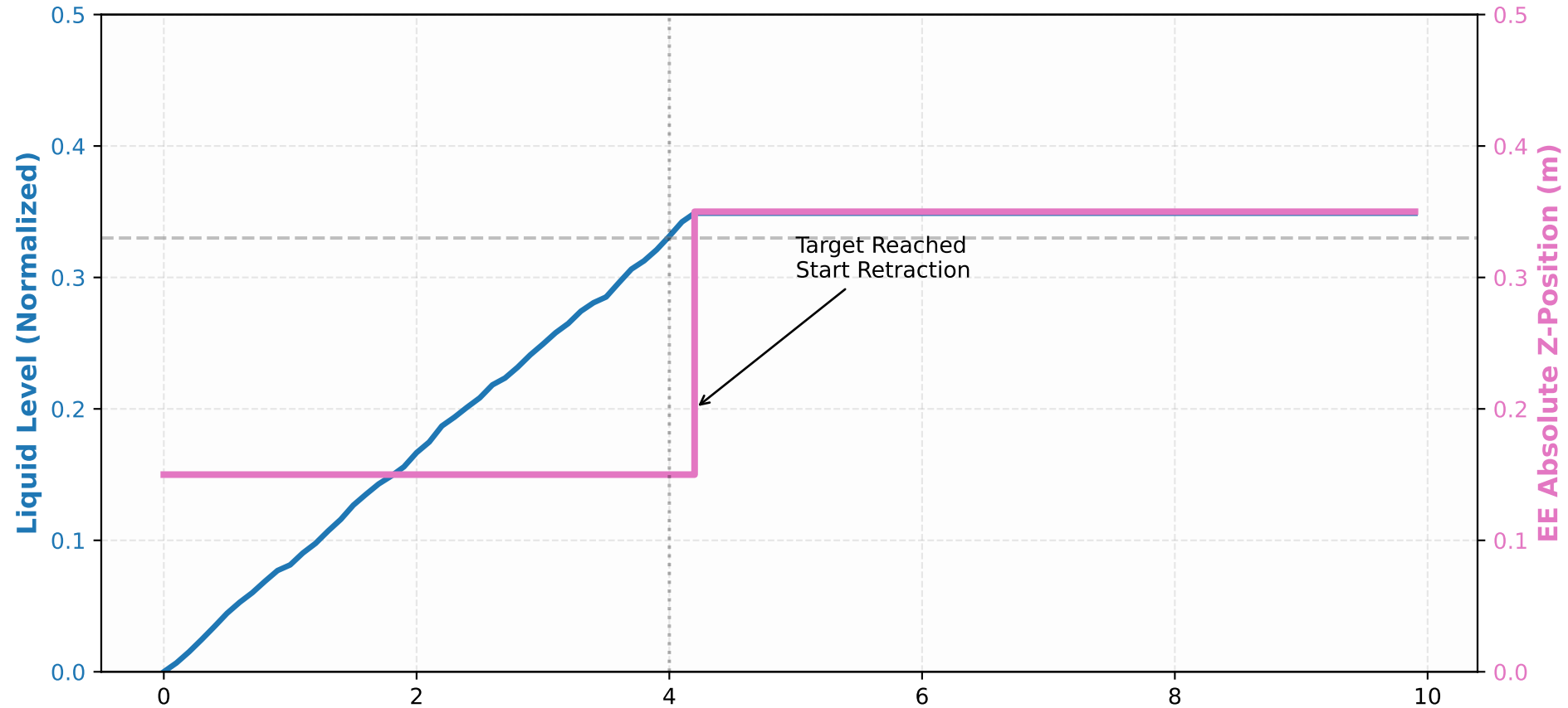
State-Action Coupling: Proportional Dispensing via Absolute Positioning
