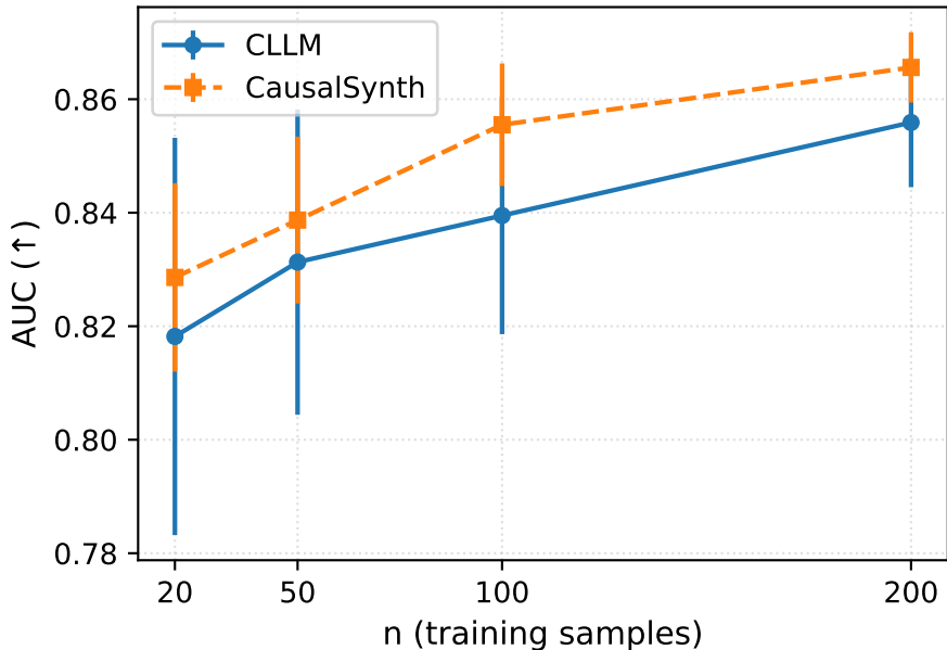
Model AUC vs. Sample Size
