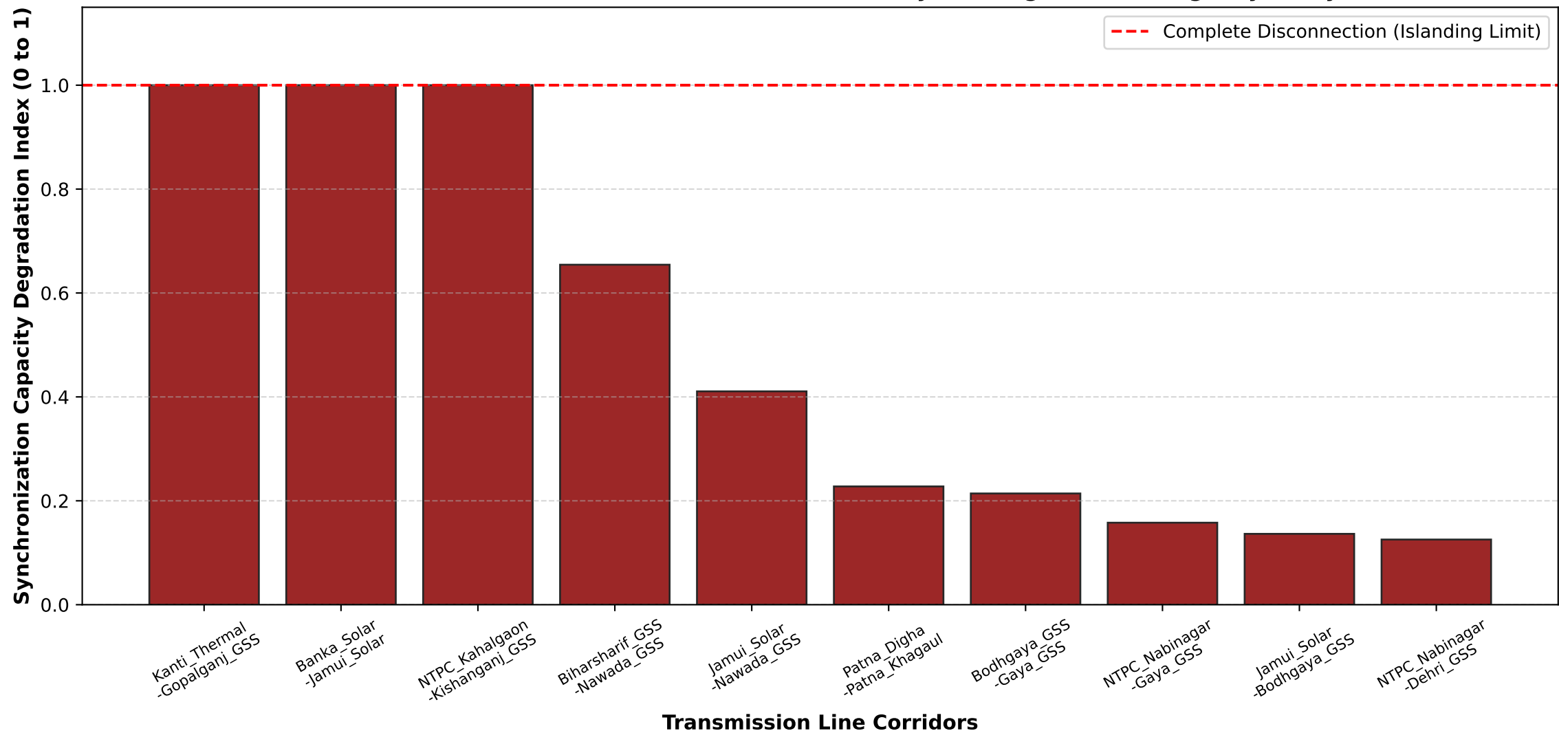
Bihar BSPTCL Grid Transmission Corridor Vulnerability Ranking (N-1 Contingency Analysis)
