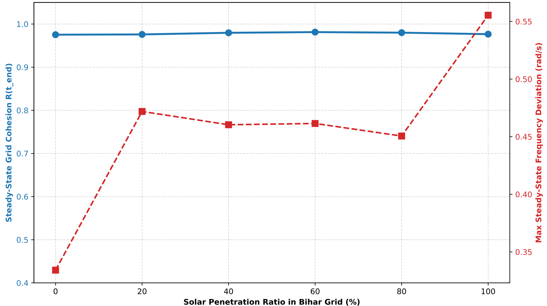
Impact of Solar Penetration on Bihar Transmission Grid Synchronization Stability
