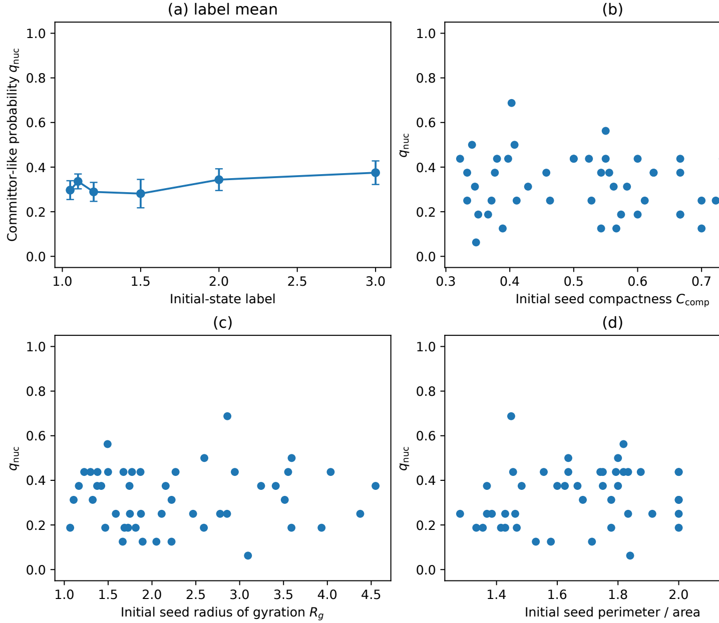
FIG. S7. Finite-time committor-style restart analysis. (a) Label-averaged restart probability q_{\text{nuc}} . (b–d) Configuration-level relations between q_{\text{nuc}} and initial seed compactness, radius of gyration, and perimeter-to-area. The weak correlations indicate that these simple scalar geometry diagnostics are not sufficient committor-level predictors in the present finite restart ensemble.
