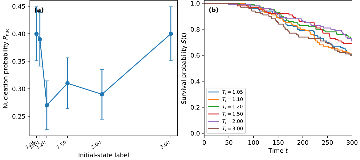
FIG. 2. Nucleation-controlled transition in the first-order \phi^6 model. (a) Nucleation probability as a function of the initial-state label. Error bars indicate standard errors over stochastic realizations. (b) Right-censored survival curves of the nucleation time. Samples that do not nucleate by the final observation time are treated as censored.
