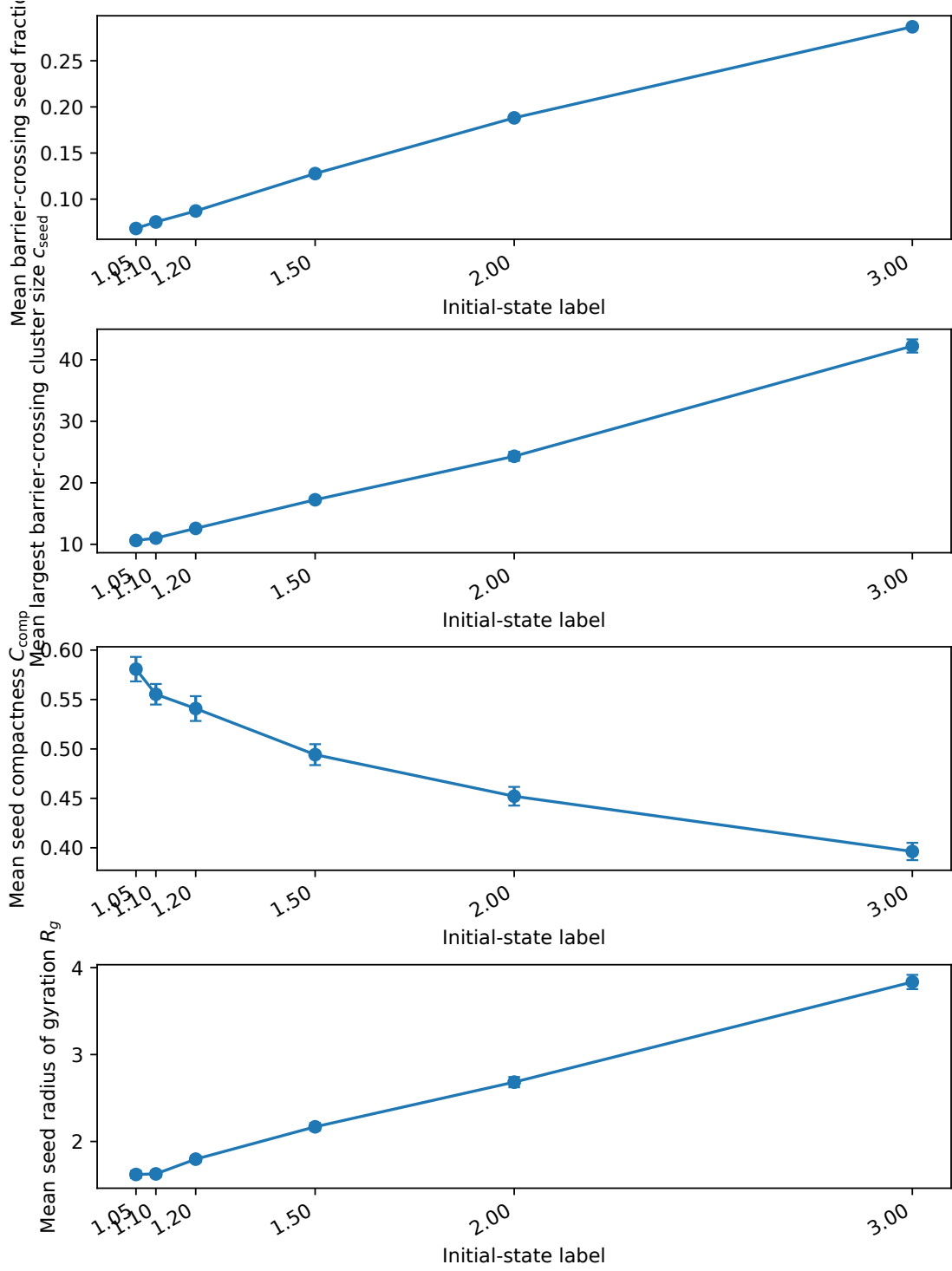
FIG. S6. Bootstrap/permutation trend-check diagnostics for the main first-order data set. The plotted observables are label means with standard-error bars. The trends in seed amount, compactness, and radius of gyration are stable under bootstrap resampling within labels.
