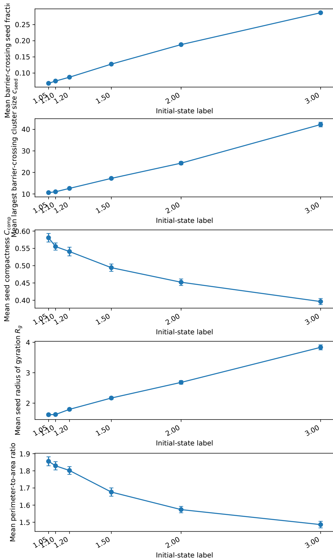
FIG. S6. Bootstrap/permutation trend-check diagnostics for the main first-order data set. The
