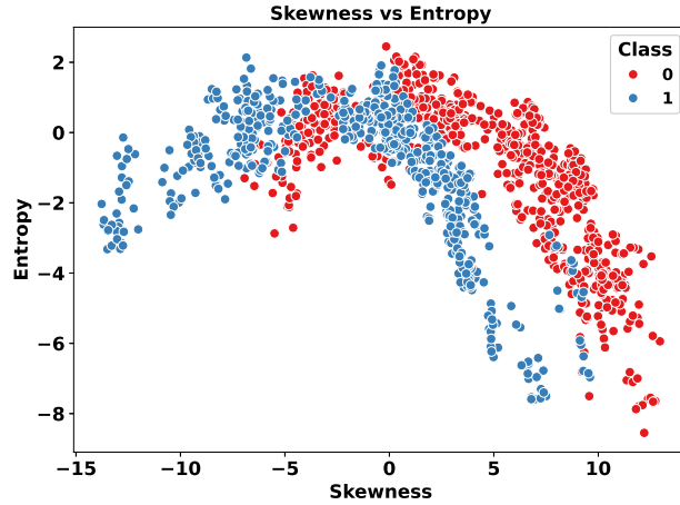
Figure 8: skewness vs entropy
