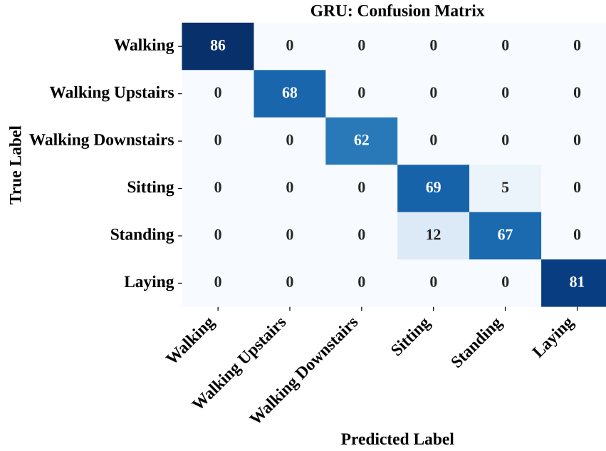
Figure 10: GRU – Confusion Matrix
