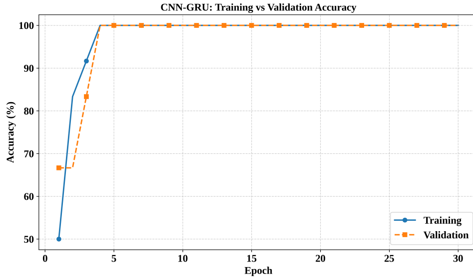
Figure 15: CNN-GRU Model – Training and Validation Accuracy
