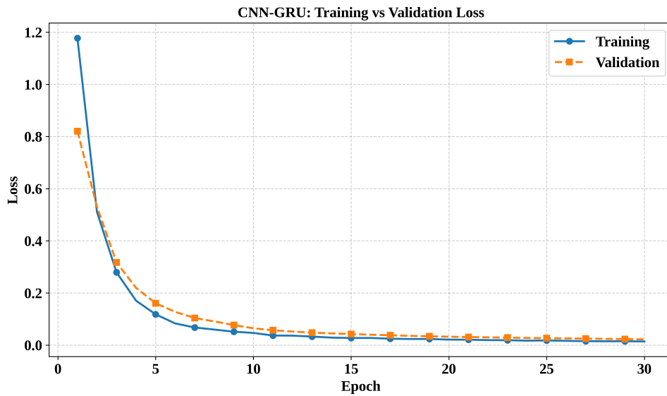
Figure 14: CNN-GRU Model – Training and Validation Loss
