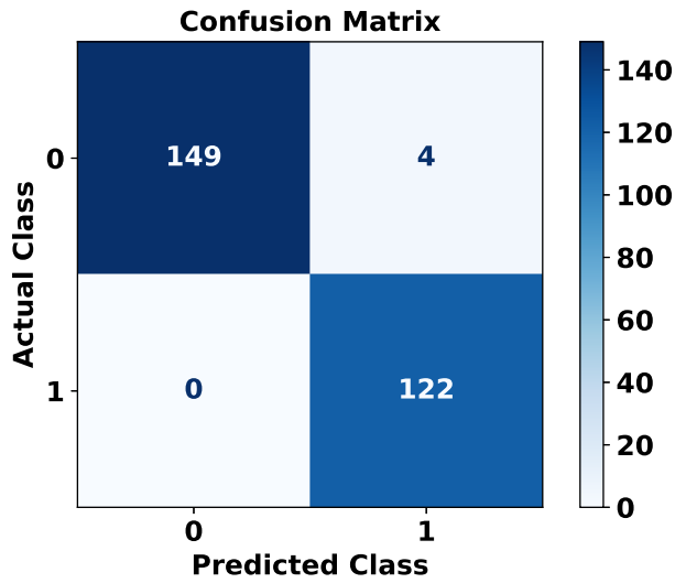
Figure 17: Confusion Matrix
