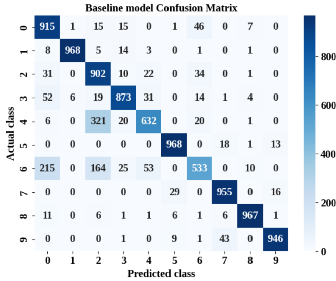
Figure 3: Baseline Model ConfusionMatrix
