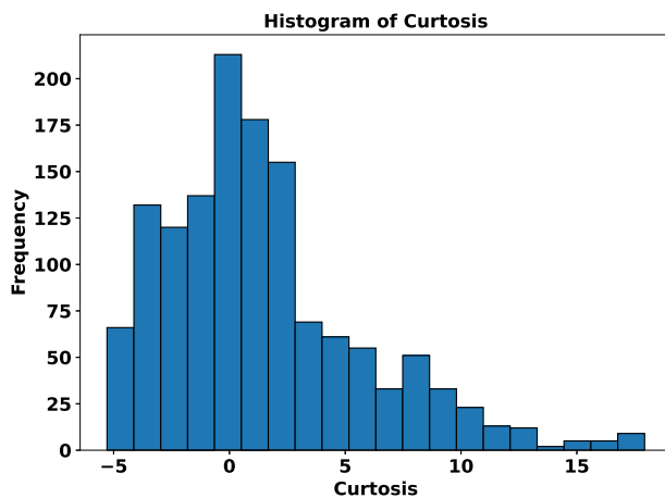
Figure 3: Histogram of Curtosis
