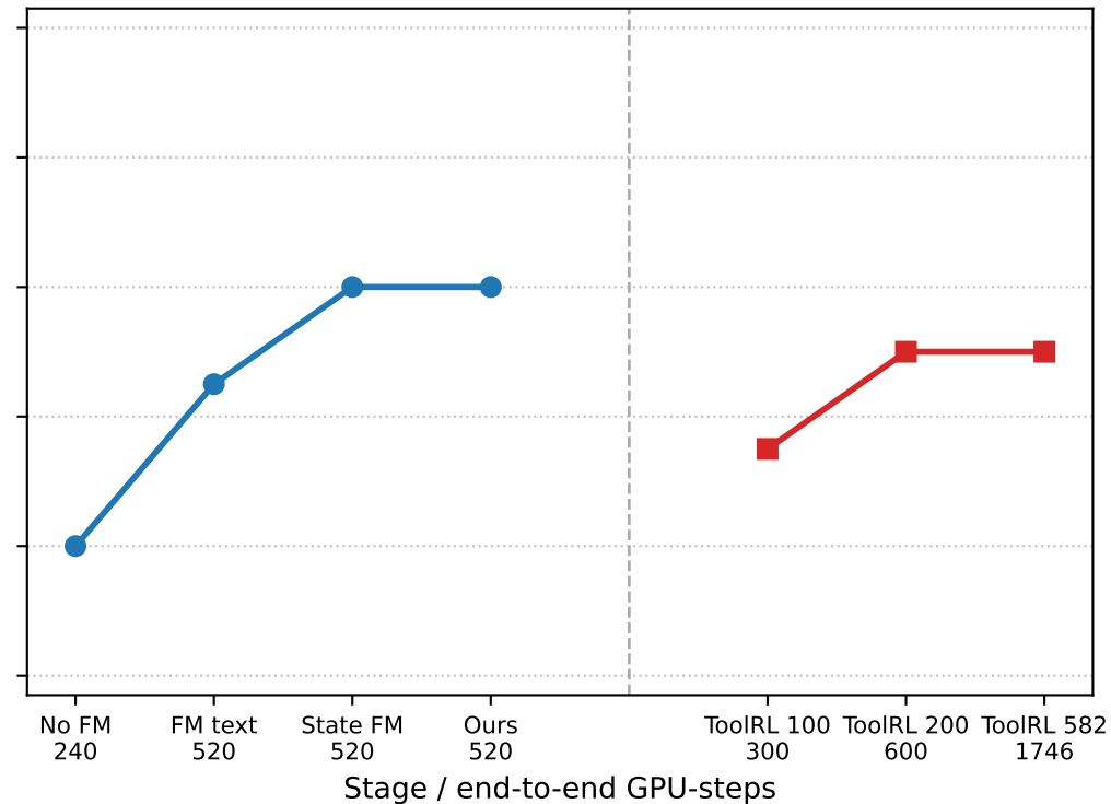
Retail success
