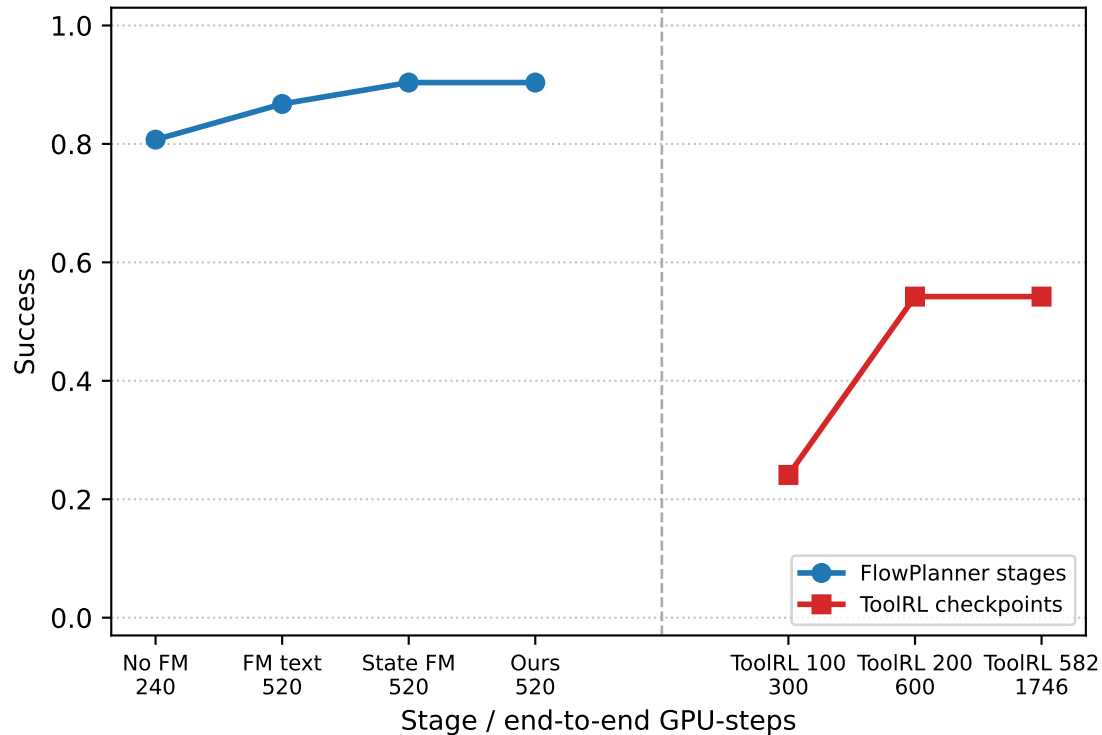
Overall success
