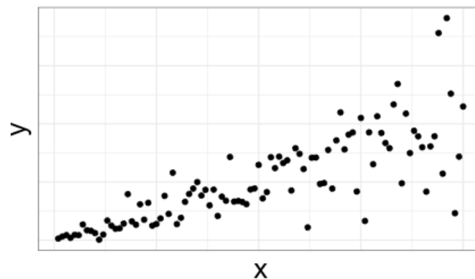
Non-constant variance
