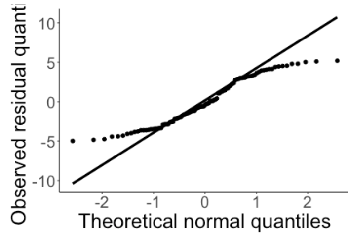
Residuals do not look normal
