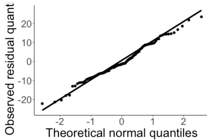
Residuals look normal
