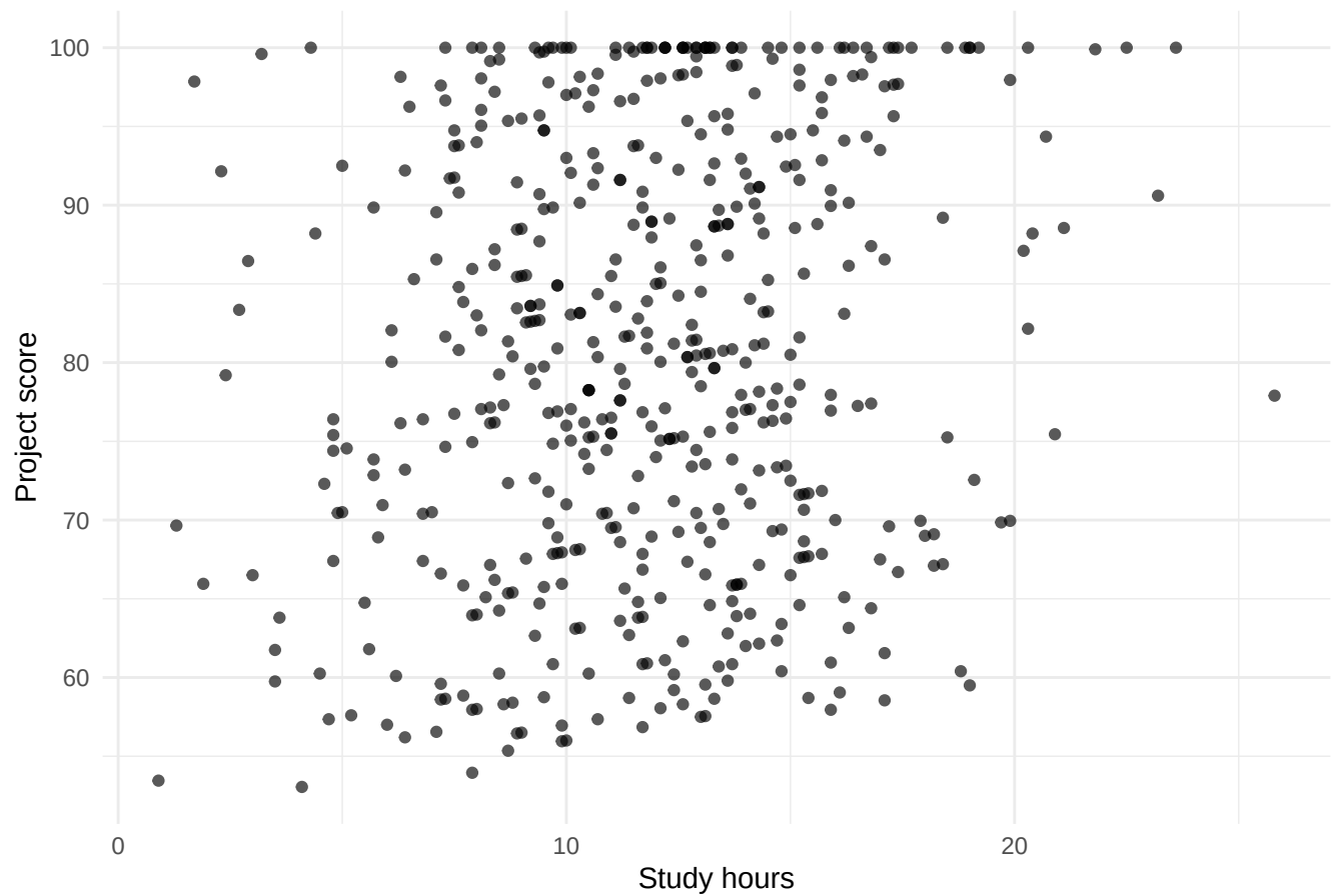
Study hours and project score
