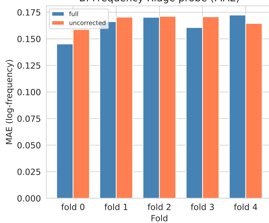
B. Frequency Ridge probe (MAE)
