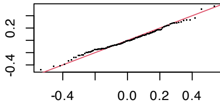
deviance residuals
