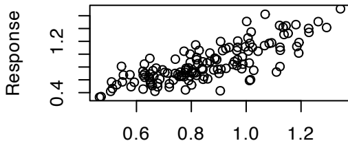
Response vs. Fitted Values
