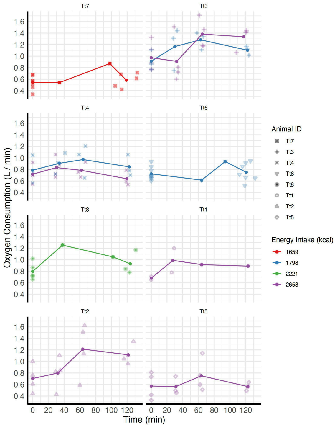
Figure S 1: Oxygen consumption as a function of time, by individual dolphin. Colors indicate energy intake in kcal. At each timepoint, varying symbols for each dolphin plot individual replicate measurements, while dots plot means at each timepoint. Nominal timepoints were 0, 30, 60, and 120 minutes, but observations are plotted at the exact time they were actually taken (or, for means, the average of those exact times).
