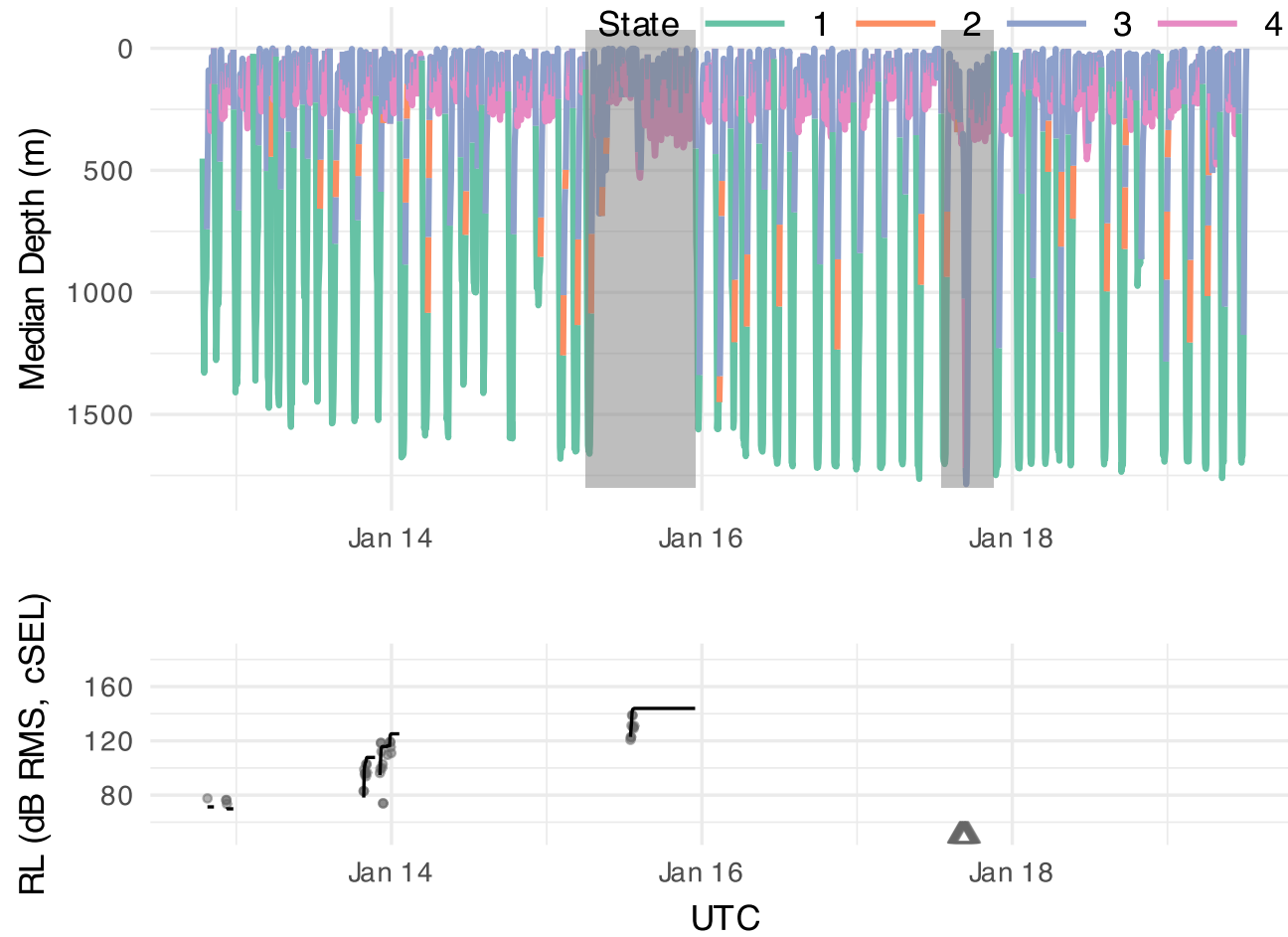
Figure S 11: Dive depth profile for tag Zica-20220112-195994, with HHMM state and sound exposure information. Open triangles indicate times orca sounds were detected on the tag record.
