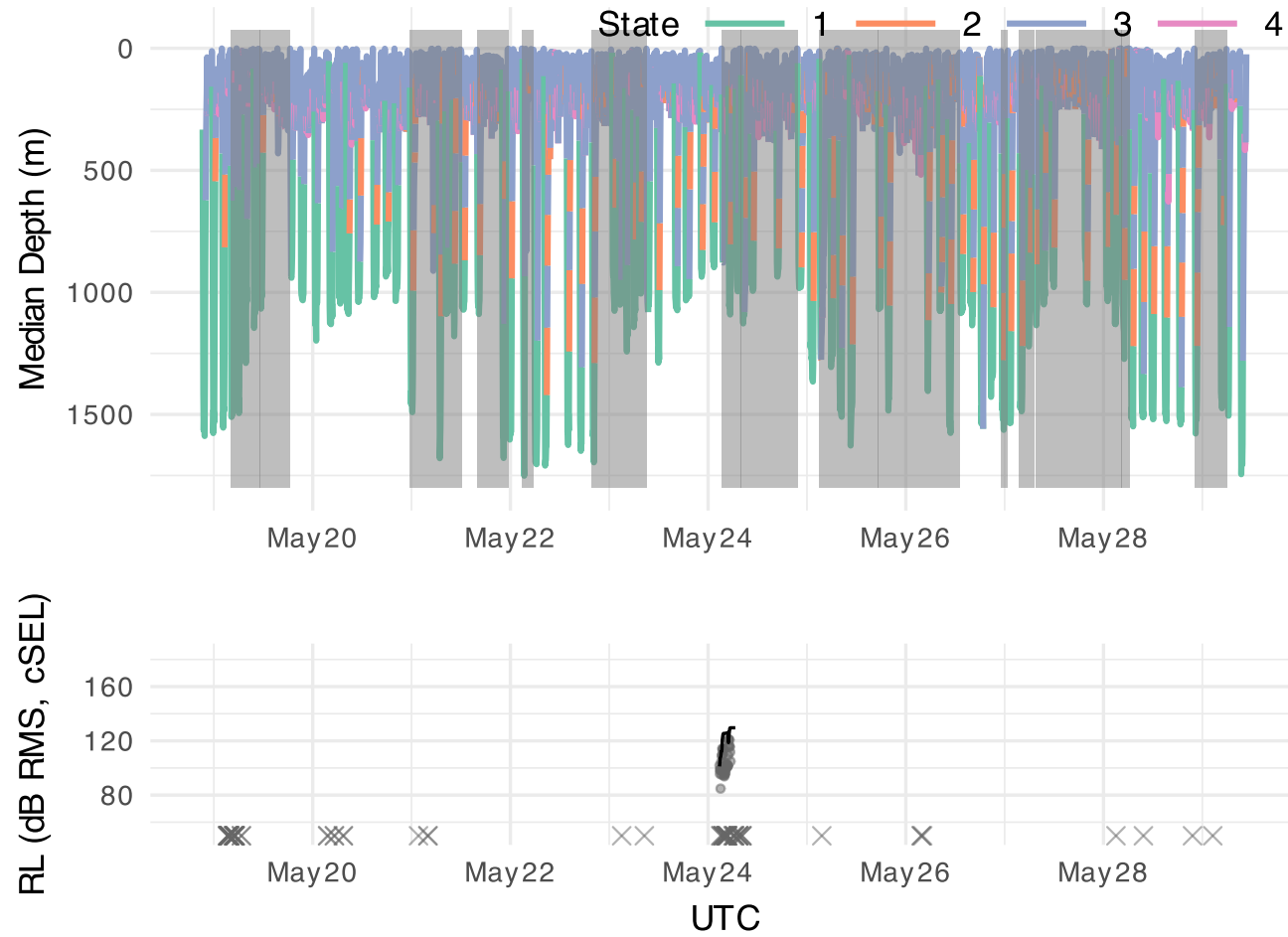
Figure S 12: Dive depth profile for tag Zica-20230518-233391, with HHMM state and sound exposure information. Xs indicate times impulsive sounds were detected on the tag record.
