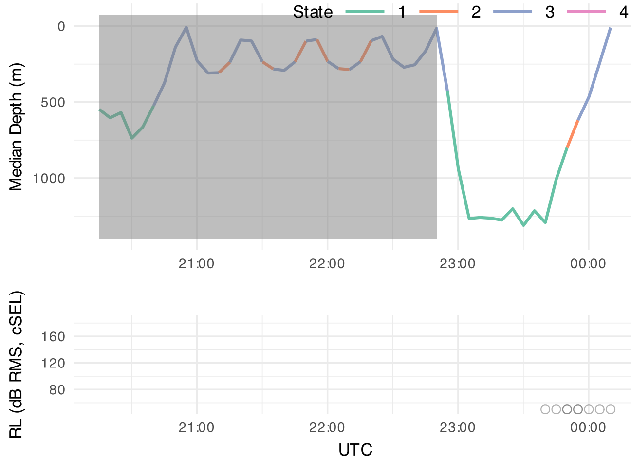
Figure S 8: Dive depth profile for tag Zica-20191117-195993, with HHMM state and sound exposure information. Open circles indicate times echosounders were detected on the tag record.
