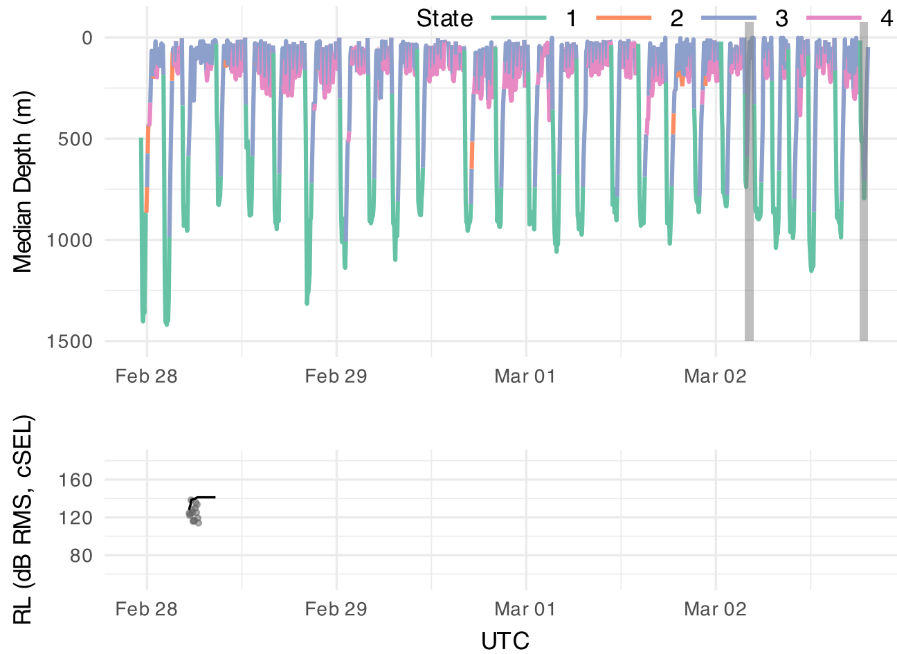
Figure S 17: Dive depth profile for tag Zica-20240227-240128, with HHMM state and sound exposure information.
