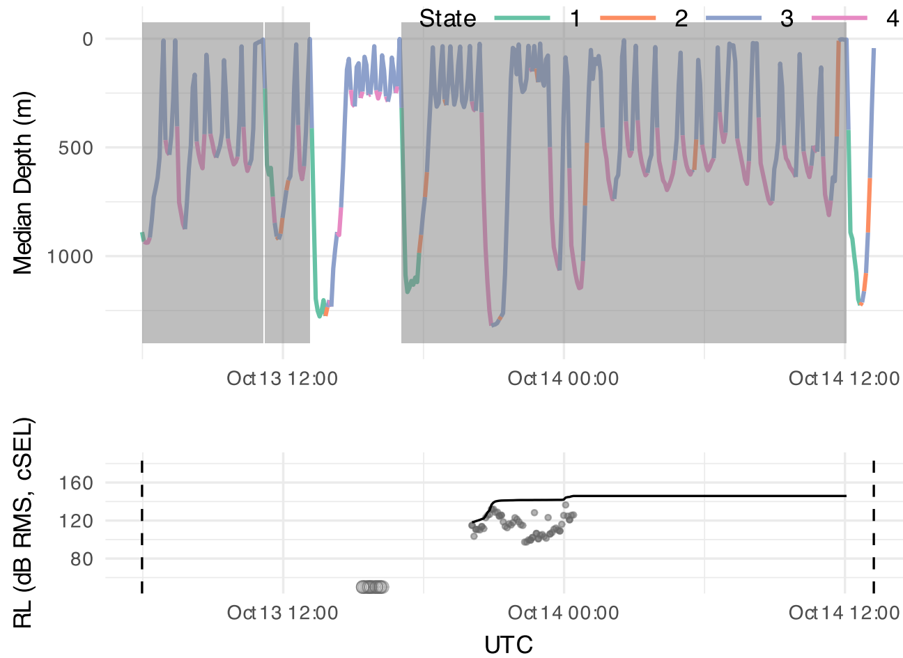
Figure S 4: Zoomed-in view of data from tag Zica-20191012-144029, from 10/13/2019 05:58 until 10/14/2019 13:14 UTC.
