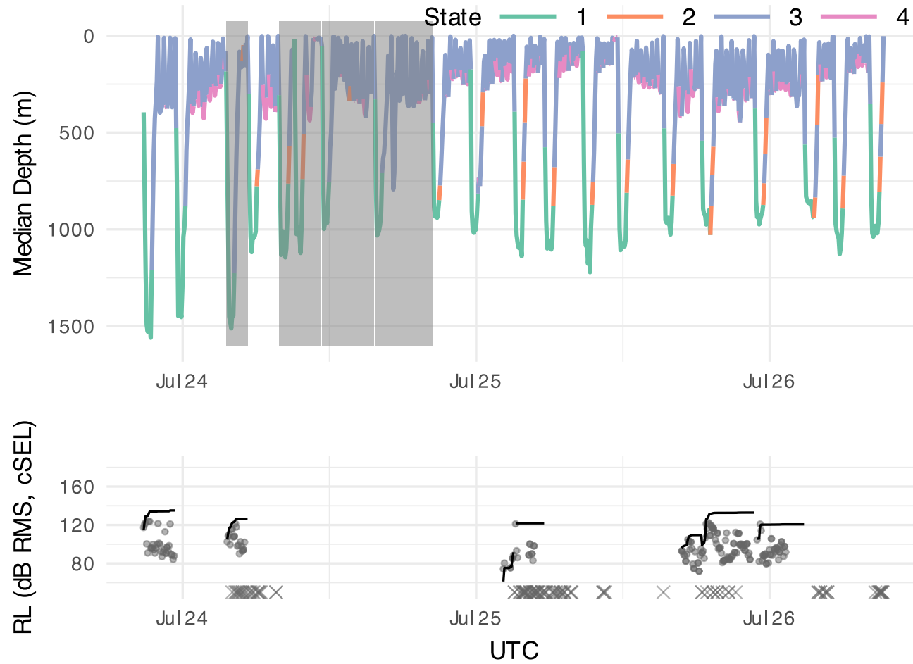
Figure S 14: Dive depth profile for tag Zica-20230723-233394, with HHMM state and sound exposure information. Xs indicate times impulsive sounds were detected on the tag record.
