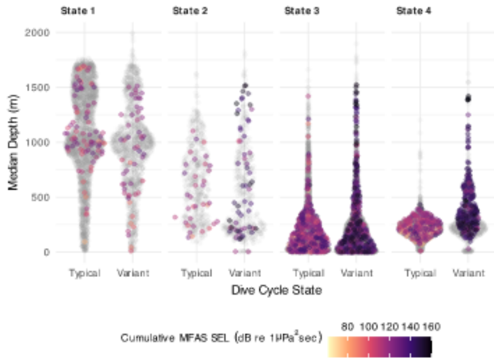
Figure S 32: Depth distribution of 5-minute intervals, by dive-cycle and 5-minute state. Color indicates MFAS cSEL.
