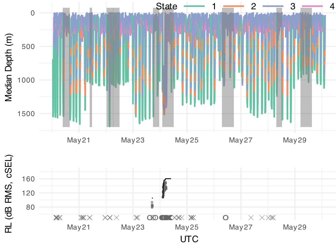
Figure S 13: Dive depth profile for tag Zica-20230519-232950, with HHMM state and sound exposure information. Symbols indicate times various sounds were detected on the tag record: open circles for echosounders and Xs for impulsive sounds.
