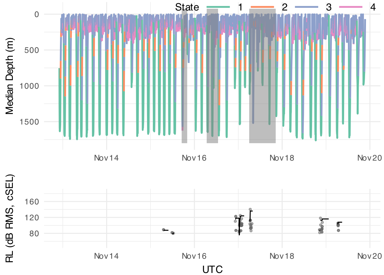
Figure S 9: Dive depth profile for tag Zica-20211112-94819, with HHMM state and sound exposure information.
