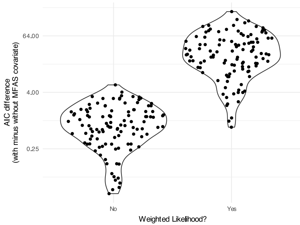
Figure S 44: By what margin would model selection using AIC select the true model ( without MFAS effect – so a small AIC difference would be hoped for), with and without duration-weighting applied to the likelihood?
