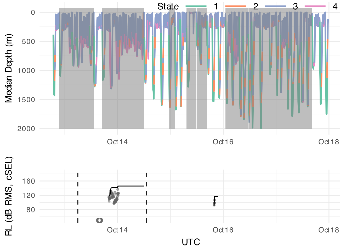
Figure S 3: Dive depth profile for tag Zica-20191012-144029, with HHMM state and sound exposure information. Open circles indicate times echosounders were detected on the tag record. Vertical dotted lines in the lower panel indicate the time-period that the next plot zooms in on.
