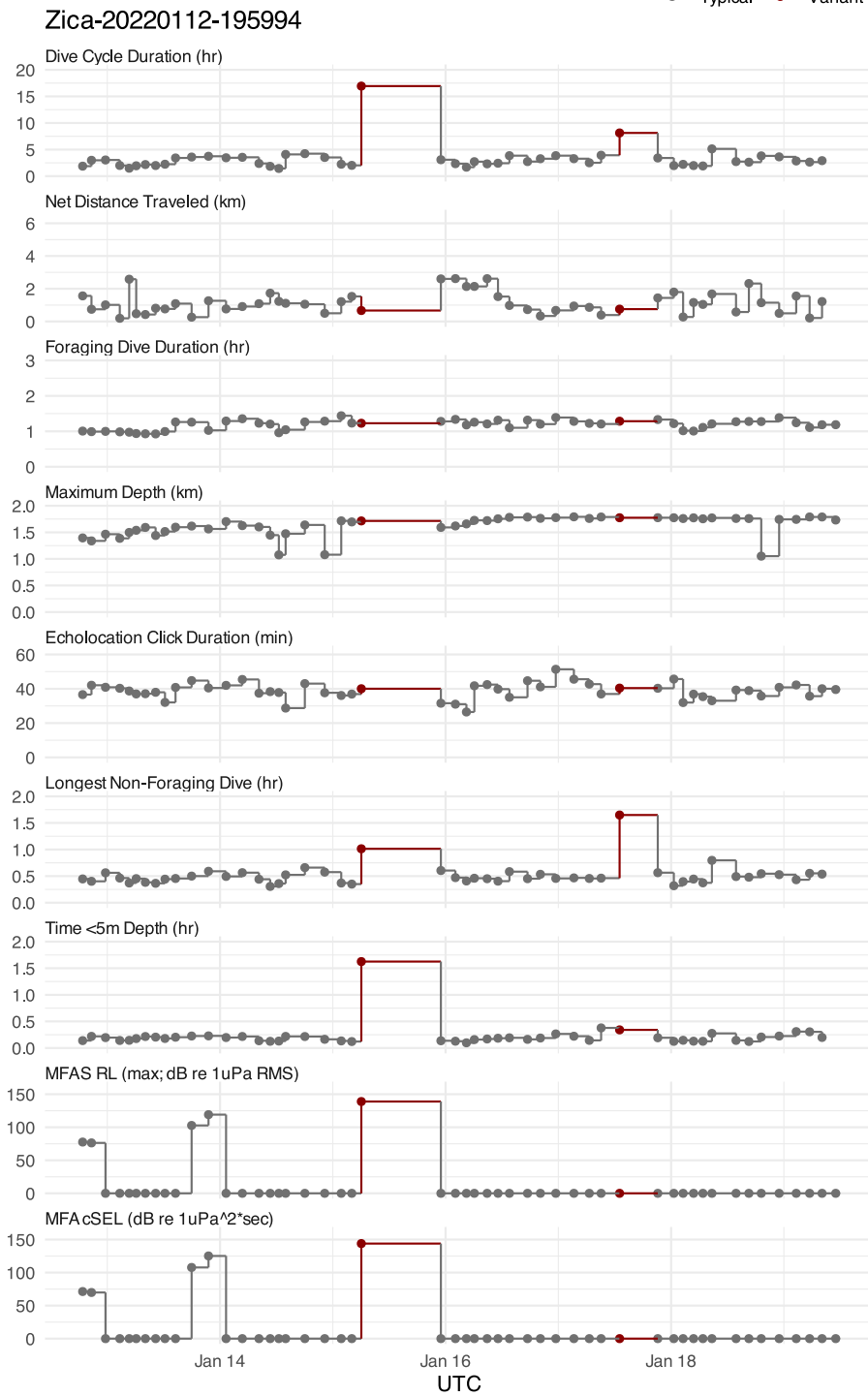
Figure S 24: HHMM input data streams for tag Zica-20220112-195994 at the dive-cycle timescale, with decoded states and MFAS exposure levels.
