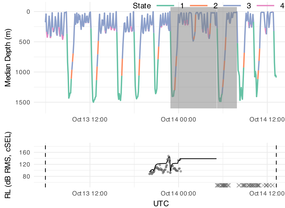
Figure S 6: Zoomed-in view of data from tag Zica-20191012-145101, from 10/13/2019 05:58 until 10/14/2019 13:14 UTC.
