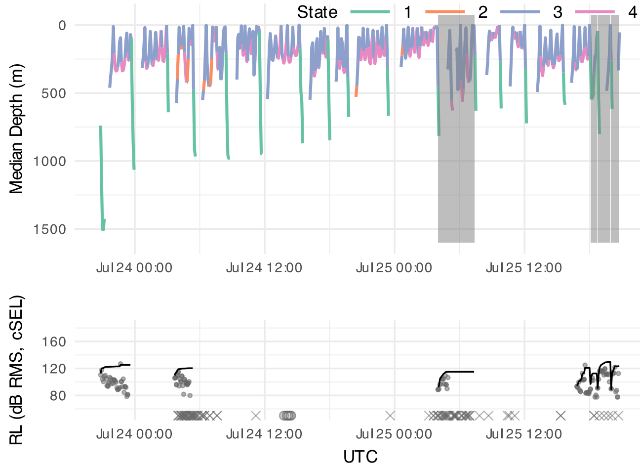
Figure S 15: Dive depth profile for tag Zica-20230723-233395, with HHMM state and sound exposure information. Symbols indicate times various sounds were detected on the tag record: open circles for echosounders and Xs for impulsive sounds.
