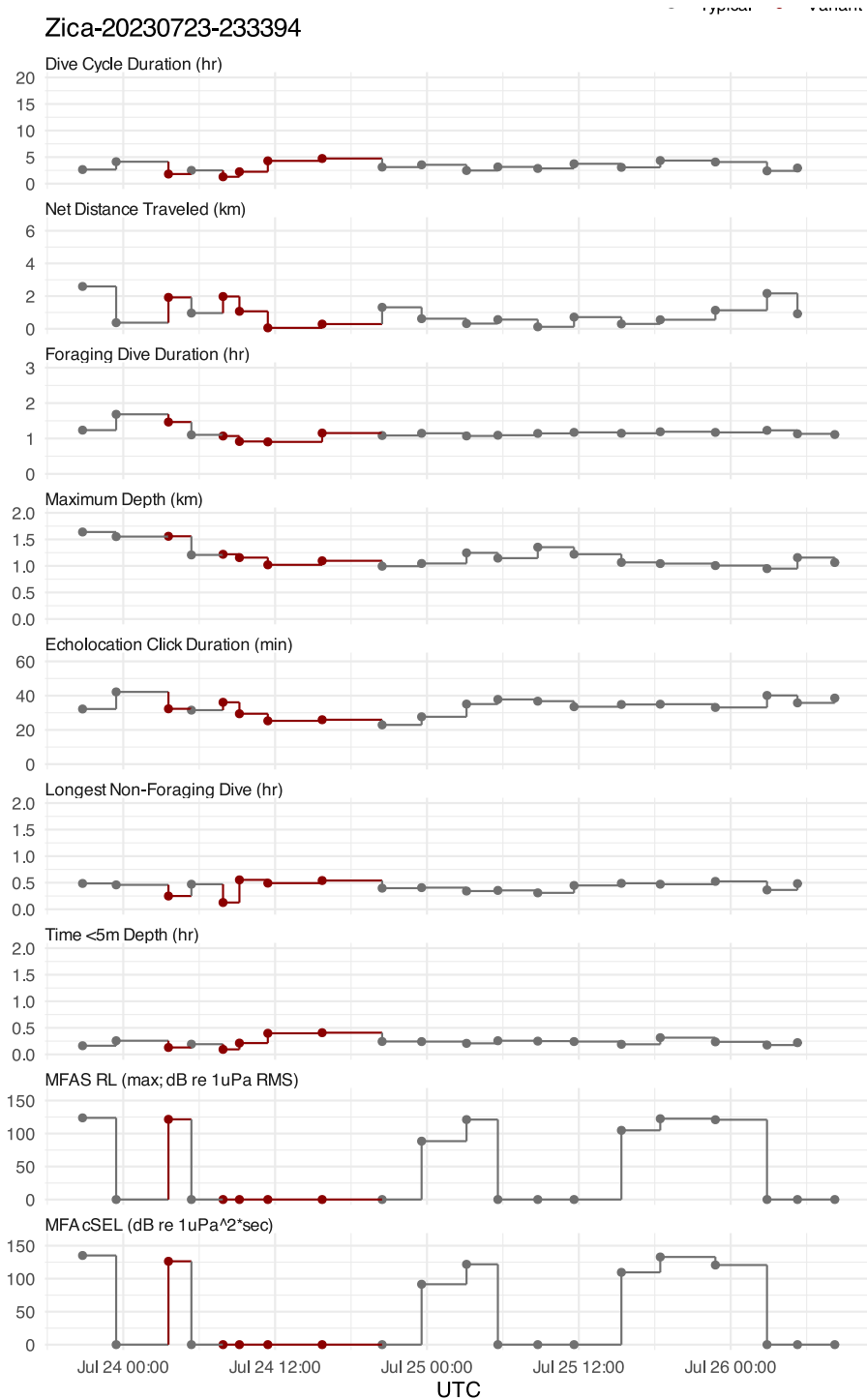
Figure S 27: HHMM input data streams for tag Zica-20230723-233394 at the dive-cycle timescale, with decoded states and MFAS exposure levels.
