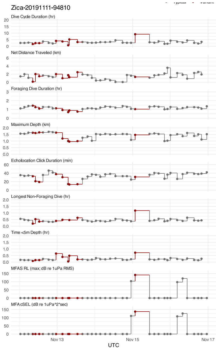
Figure S 20: HHMM input data streams for tag Zica-20191111-94810 at the dive-cycle timescale, with decoded states and MFAS exposure levels.
