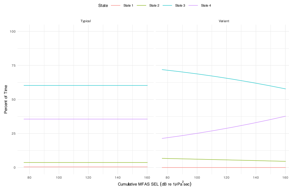
Figure S 36: Stationary state distribution at the dive-cycle scale. The values show the expected proportion of dive cycles spent in each state if the MFAS exposure level was perpetually at a certain value.
