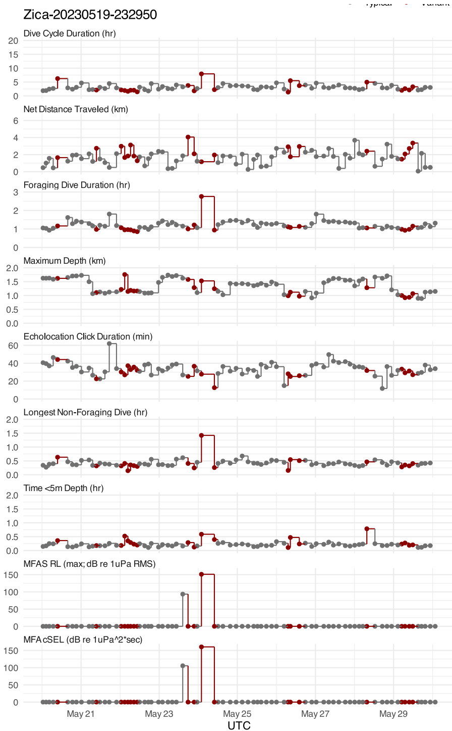
Figure S 26: HHMM input data streams for tag Zica-20230519-232950 at the dive-cycle timescale, with decoded states and MFAS exposure levels.
