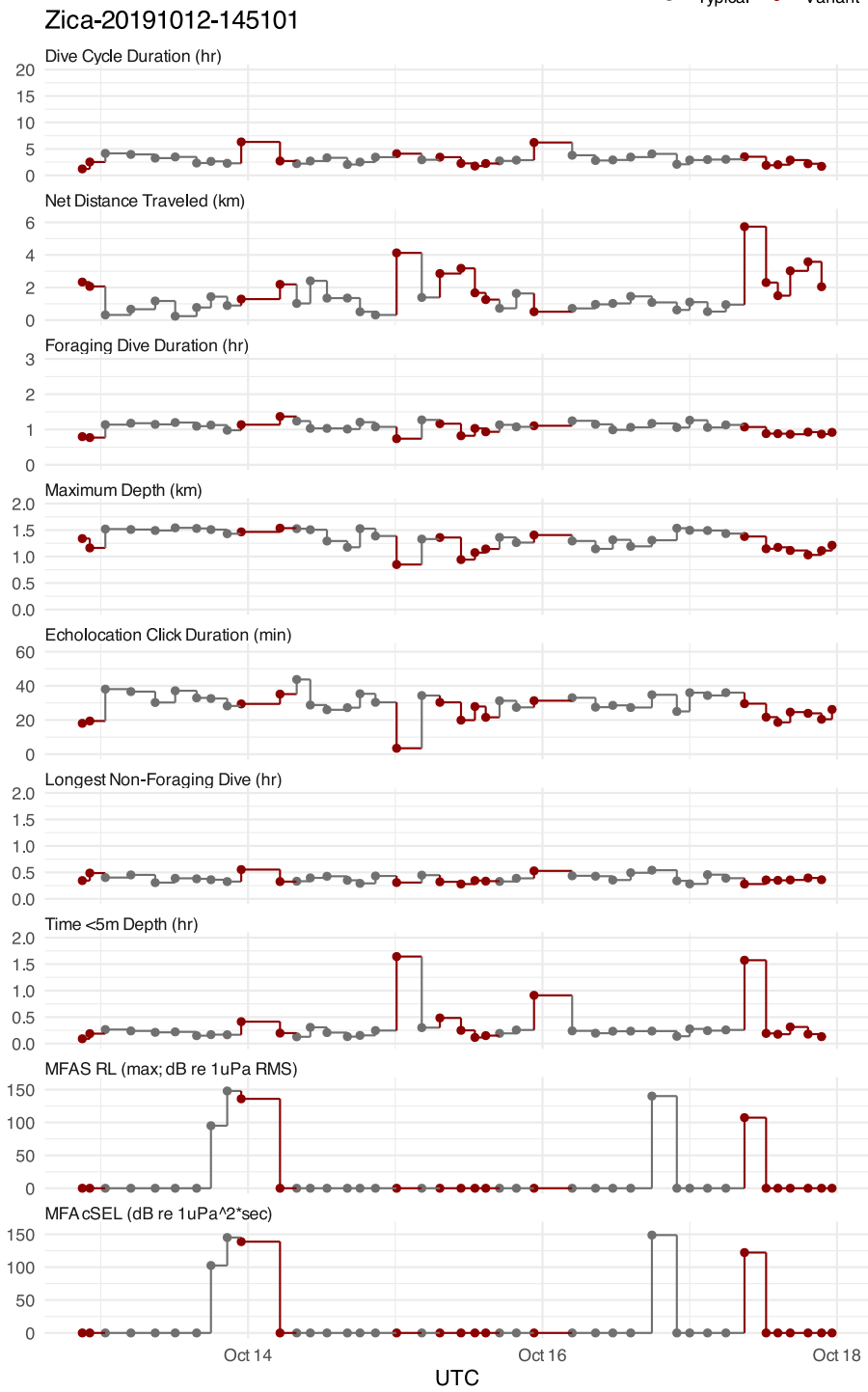
Figure S 19: HHMM input data streams for tag Zica-20191012-145101 at the dive-cycle timescale, with decoded states and MFAS exposure levels.
