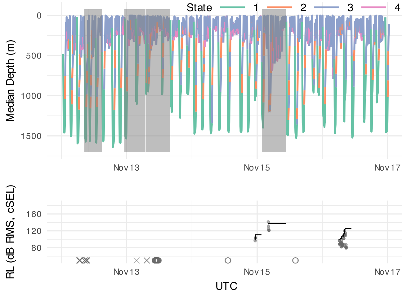
Figure S 7: Dive depth profile for tag Zica-20191111-94810, with HHMM state and sound exposure information. Symbols indicate times various sounds were detected on the tag record: open circles for echosounders and Xs for impulsive sounds.
