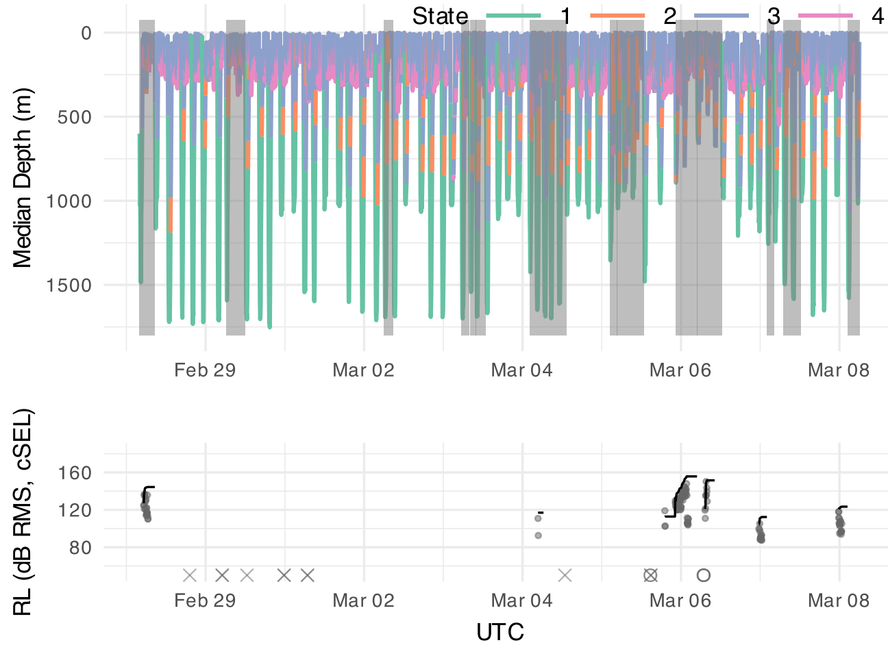
Figure S 16: Dive depth profile for tag Zica-20240227-233396, with HHMM state and sound exposure information. Symbols indicate times various sounds were detected on the tag record: open circles for echosounders and Xs for impulsive sounds.
