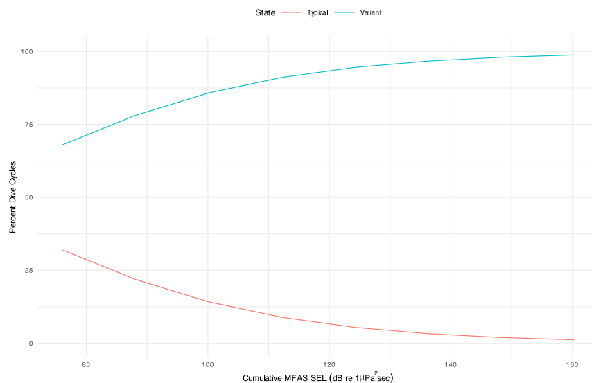
Figure S 35: Stationary state distribution at the dive-cycle scale. The values show the expected proportion of dive cycles spent in each state if the MFAS exposure level was perpetually at a certain value.
