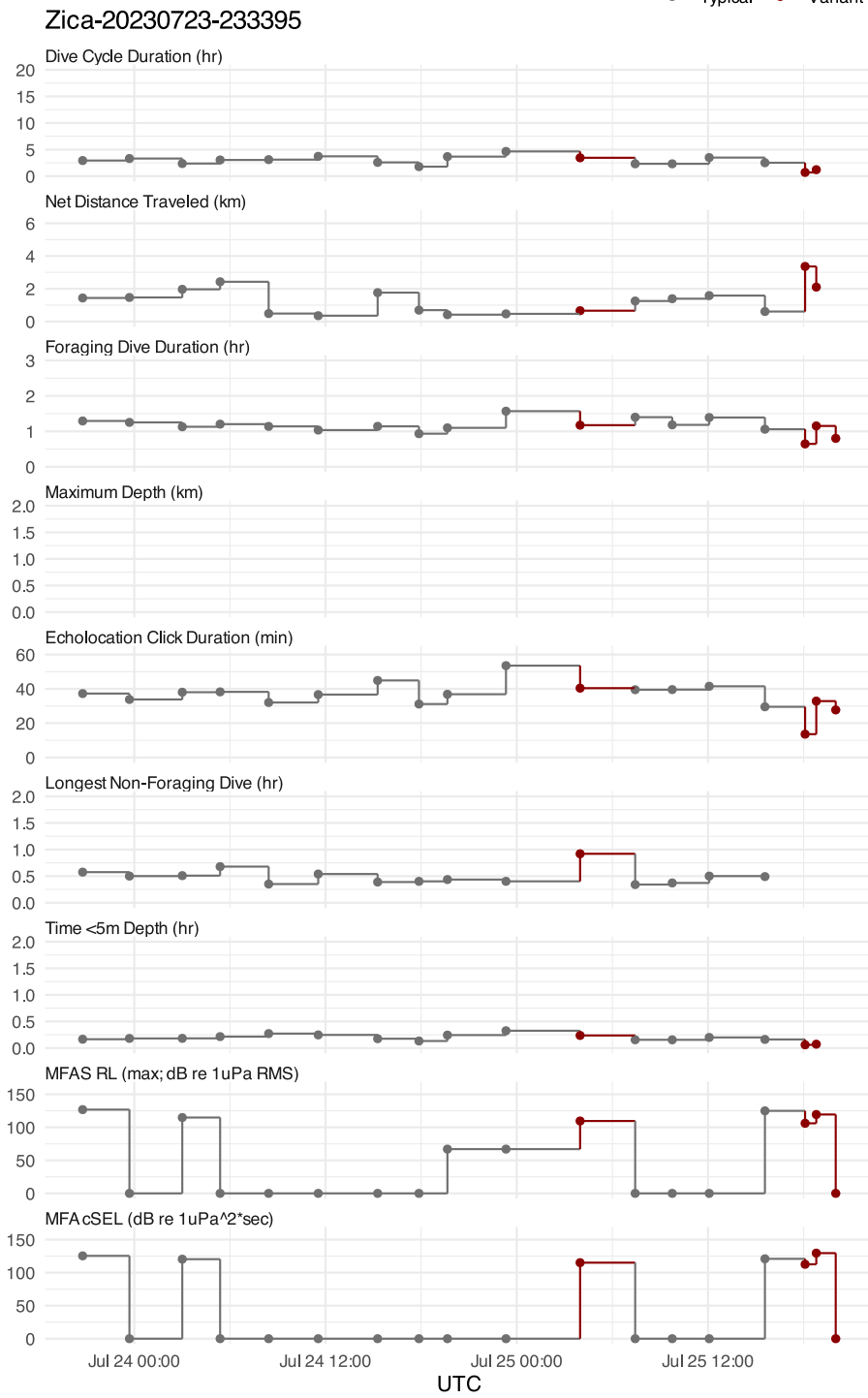
Figure S 28: HHMM input data streams for tag Zica-20230723-233395 at the dive-cycle timescale, with decoded states and MFAS exposure levels.
