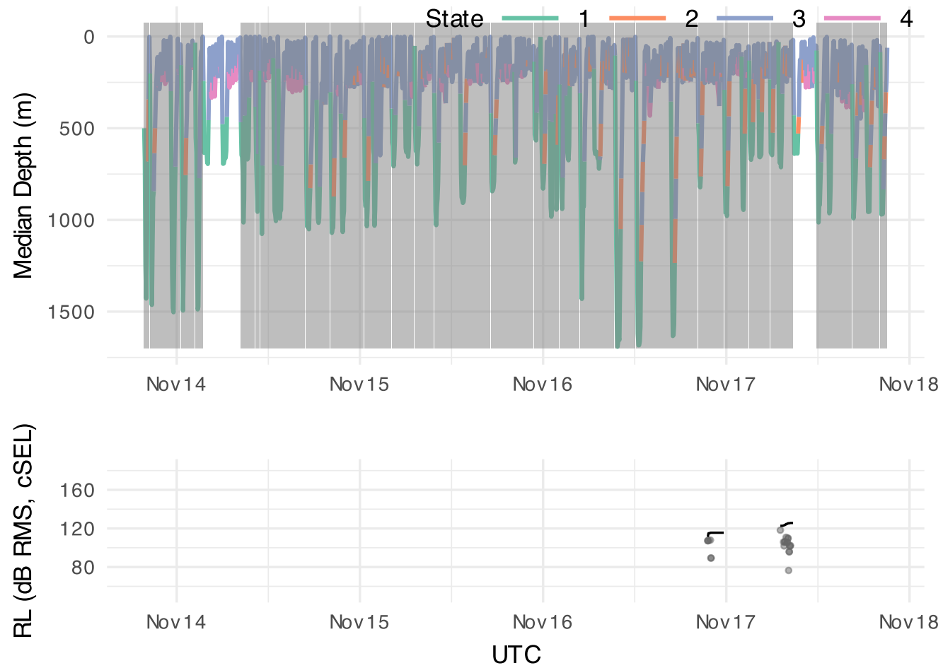
Figure S 10: Dive depth profile for tag Zica-20211113-195993, with HHMM state and sound exposure information.
