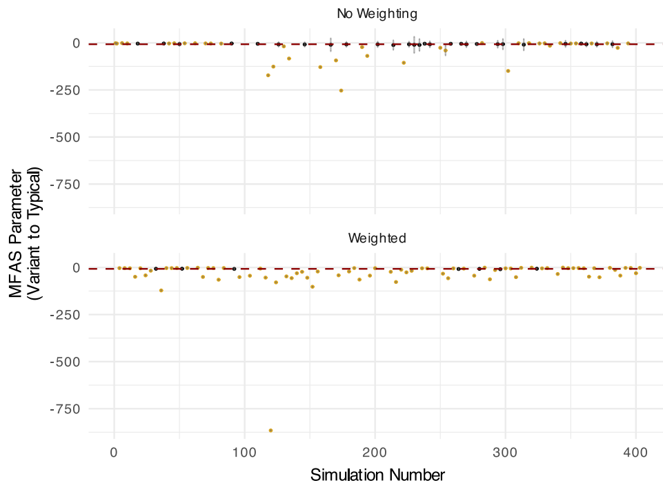
Figure S 43: Parameter estimates and 95% confidence intervals for the parameter measuring the effect of MFAS on transition from Variant to Typical state (note, this one is not estimated well because of the small size of the dataset). Dotted horizontal line shown the true value of the parameter.
