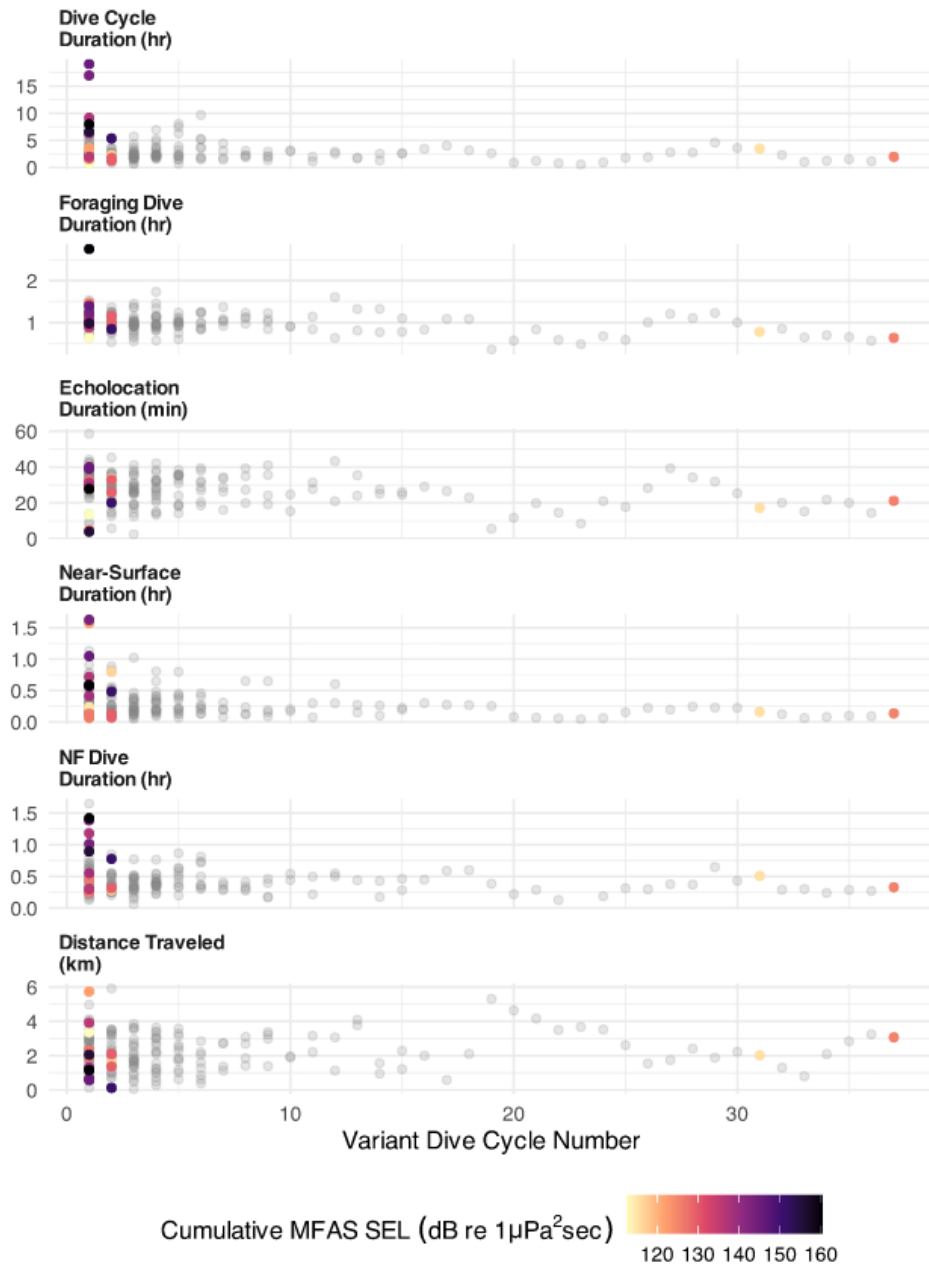
Figure S 31: Dive-cycle characteristics of variant dive cycles as a function of dive-cycle number, within the sequence of several variant dive cycles.
