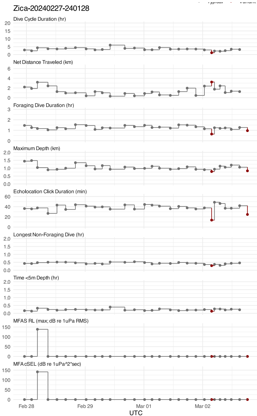
Figure S 30: HHMM input data streams for tag Zica-20240227-240128 at the dive-cycle timescale, with decoded states and MFAS exposure levels.
