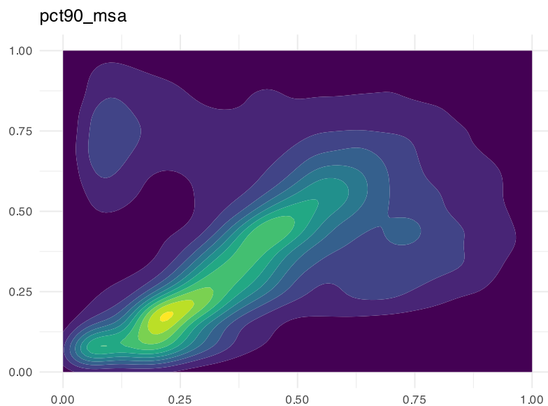
Figure S 37: Lag plot for 90th percentile of MSA.
