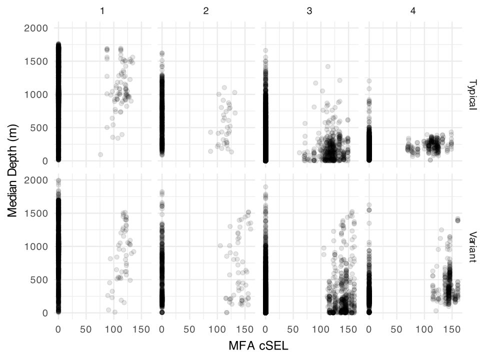
Figure S 33: Depth as a function of MFAS cSEL for 5-minute intervals, by dive-cycle and 5-minute state.
