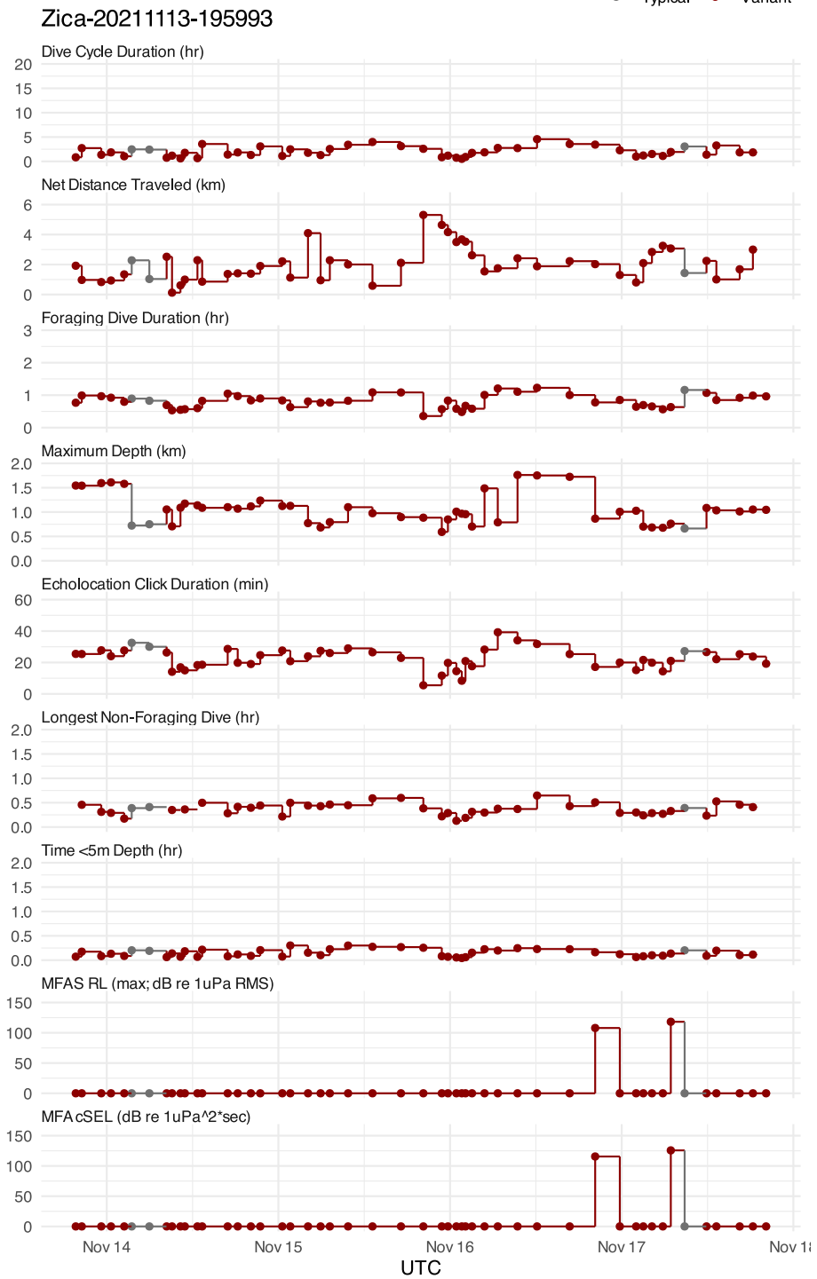
Figure S 23: HHMM input data streams for tag Zica-20211113-195993 at the dive-cycle timescale, with decoded states and MFAS exposure levels.
