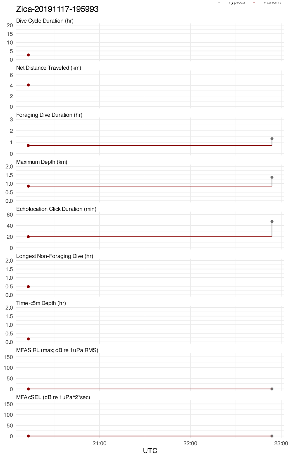
Figure S 21: HHMM input data streams for tag Zica-20191117-195993 at the dive-cycle timescale, with decoded states and MFAS exposure levels.
