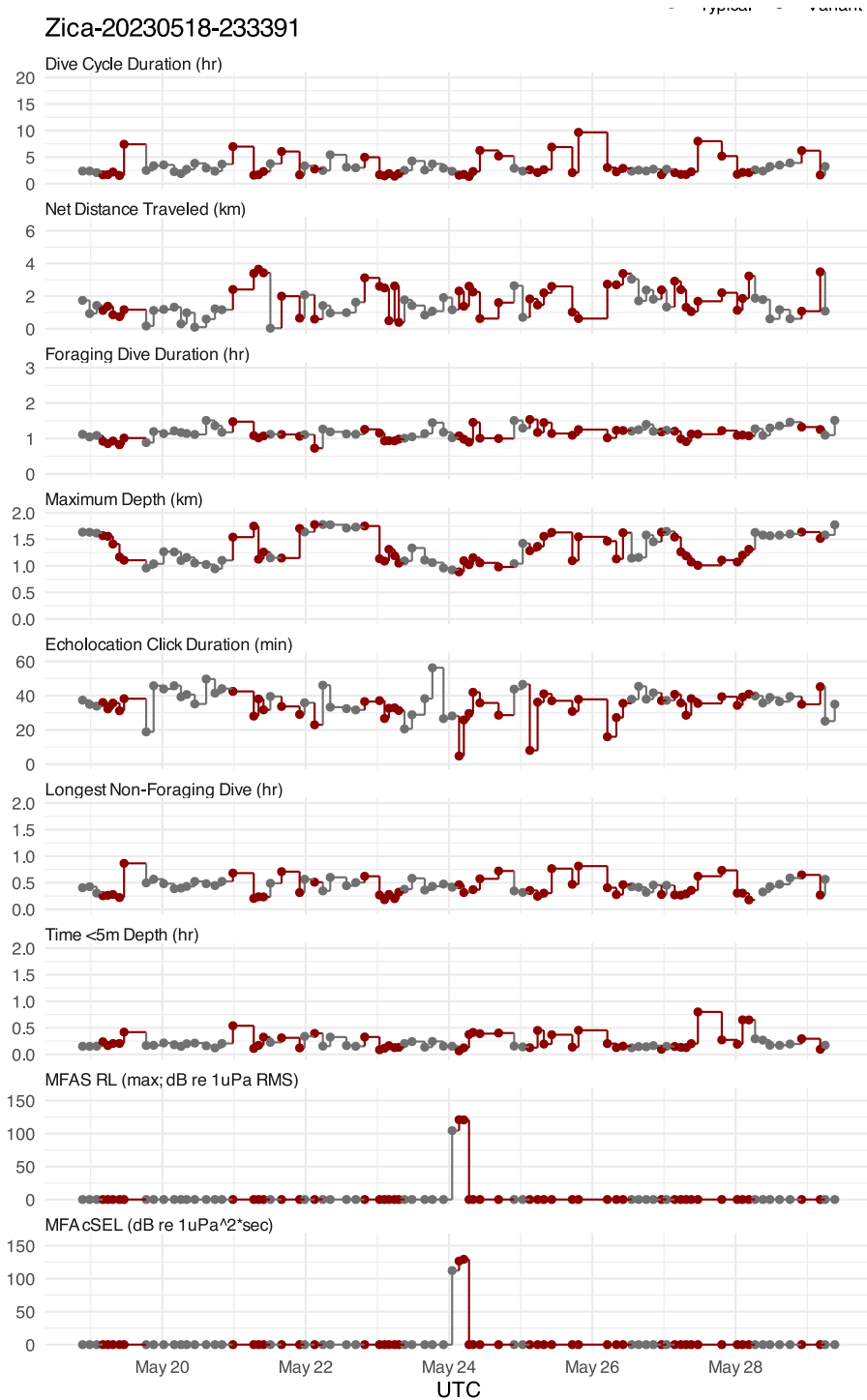
Figure S 25: HHMM input data streams for tag Zica-20230518-233391 at the dive-cycle timescale, with decoded states and MFAS exposure levels.
