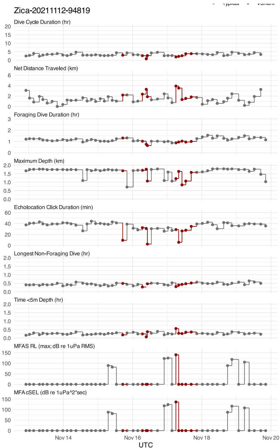
Figure S 22: HHMM input data streams for tag Zica-20211112-94819 at the dive-cycle timescale, with decoded states and MFAS exposure levels.
