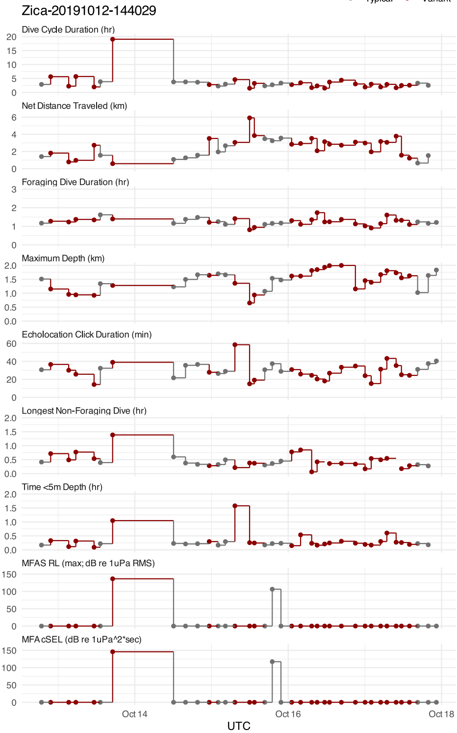
Figure S 18: HHMM input data streams for tag Zica-20191012-144029 at the dive-cycle timescale, with decoded states and MFAS exposure levels.
