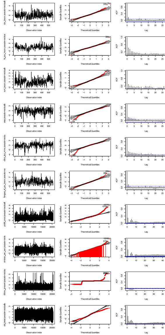
Figure S 40: HHMM pseudo-residuals.
