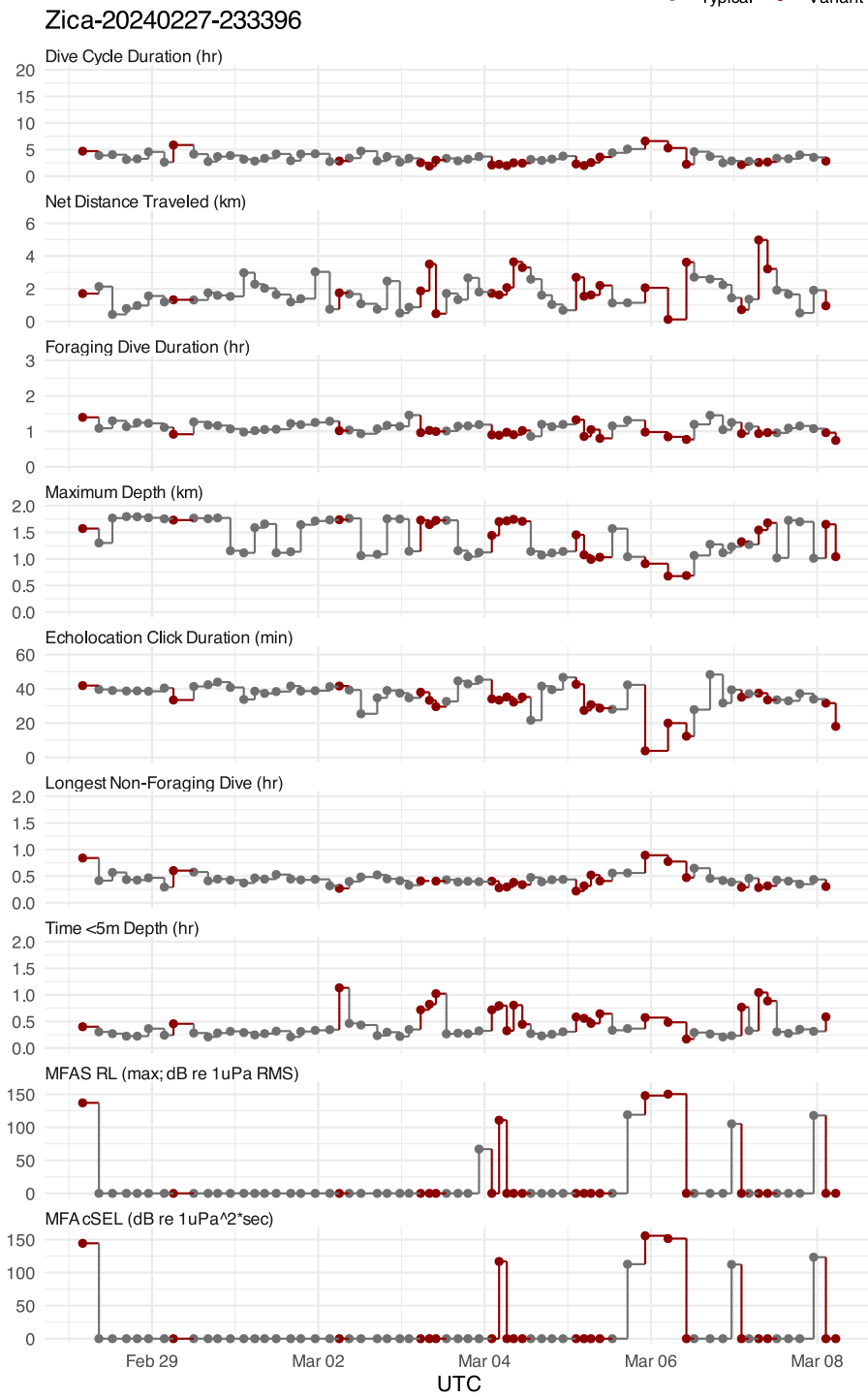
Figure S 29: HHMM input data streams for tag Zica-20240227-233396 at the dive-cycle timescale, with decoded states and MFAS exposure levels.
