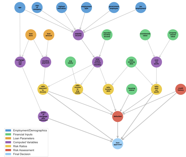
Figure 3: Diagram of the 27-node LGBN
