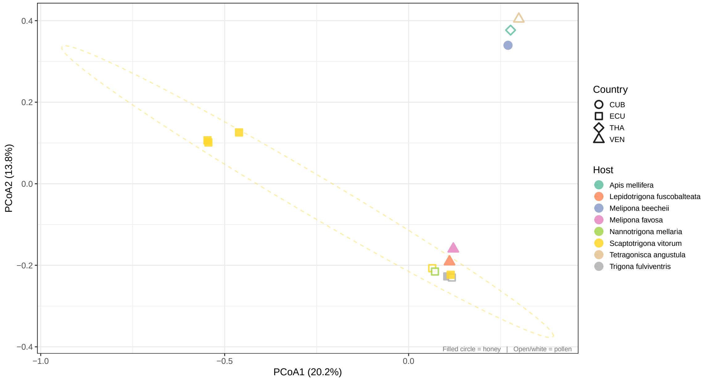
ITS PCoA JACCARD
