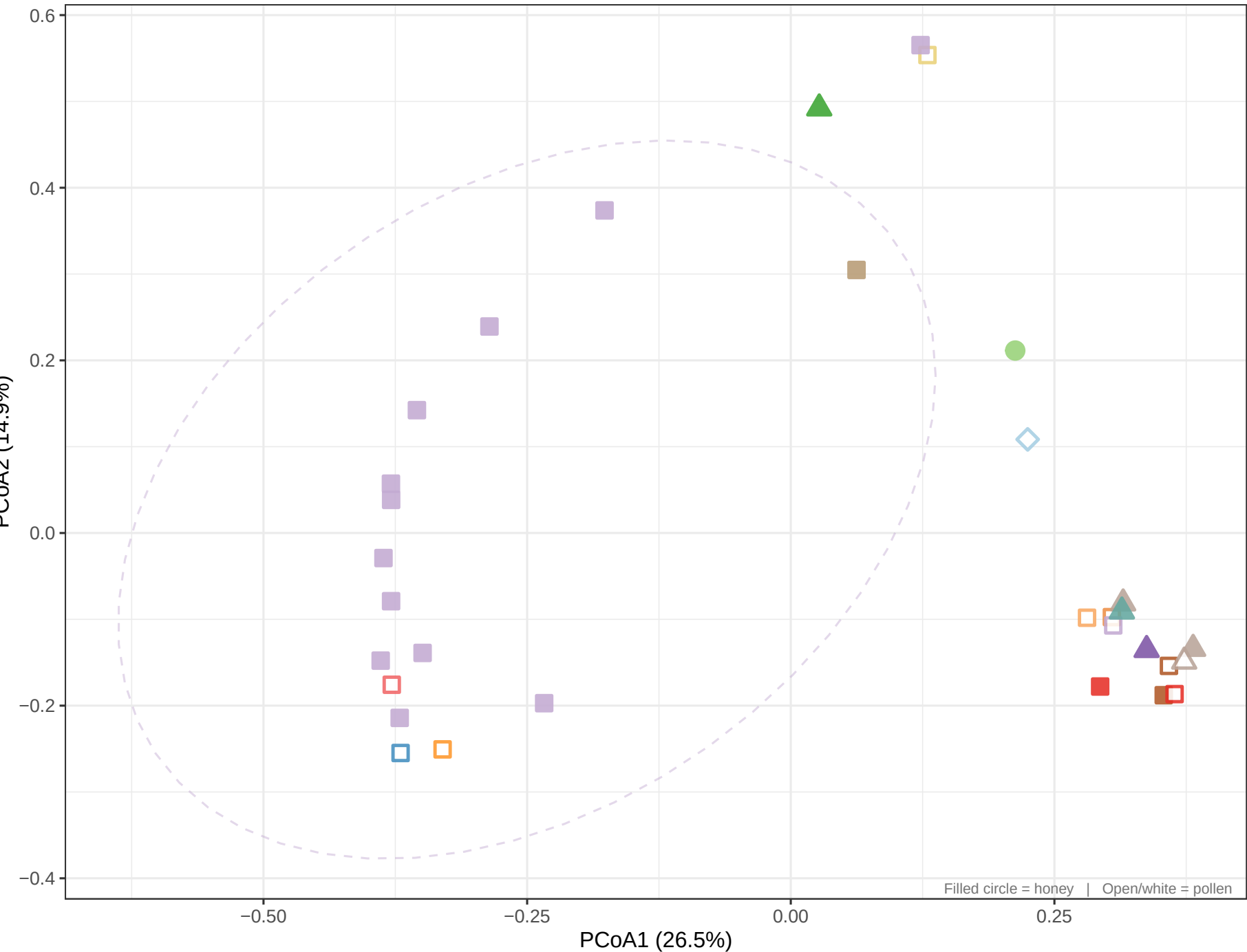
16S PCoA BRAY
