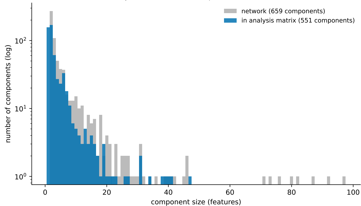
Molecular-family sizes shrink once isotope/adduct/ISF rows are removed
