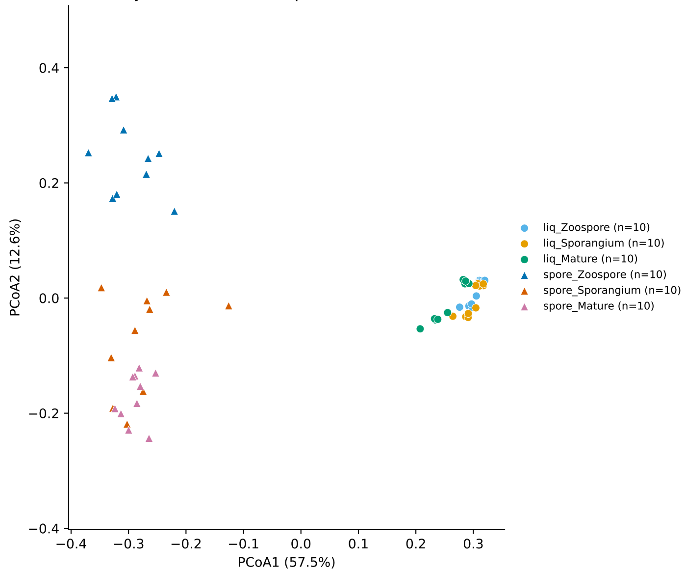
Bray-Curtis PCoA -- sampled condition (n=60)
