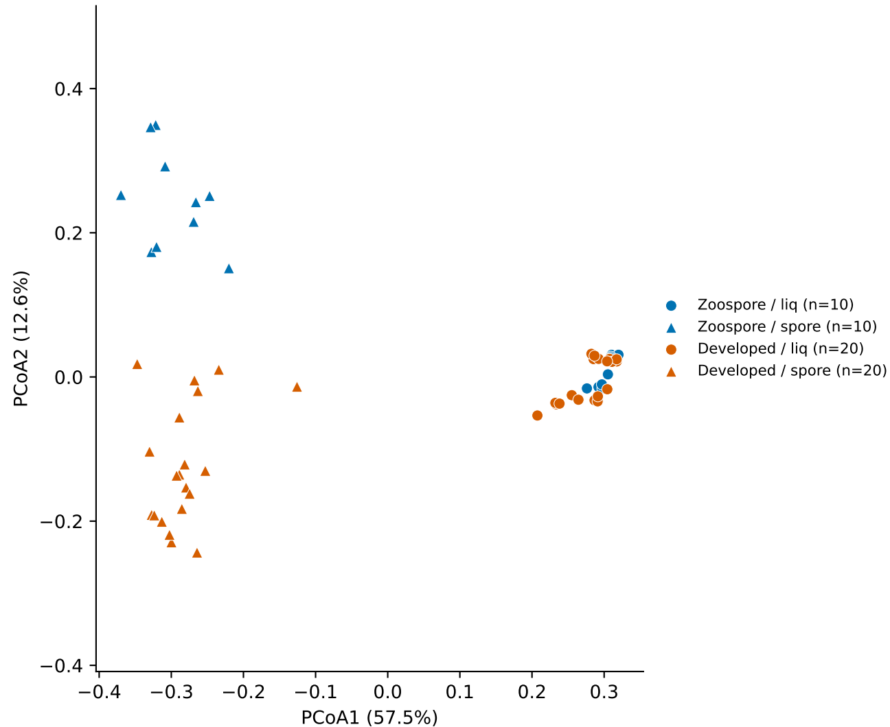
Bray-Curtis PCoA -- Zoospore vs Developed (n=60)
