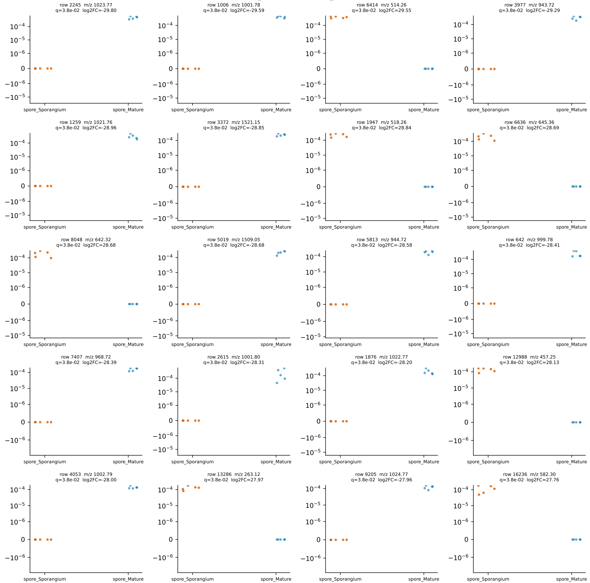
Top 20 differential features: spore_Sporangium vs spore_Mature (TSS proportion, symlog y)
