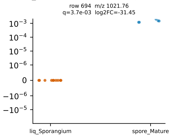
Top 20 differential features: liq_Sporangium vs spore_Mature (TSS proportion, symlog y)
