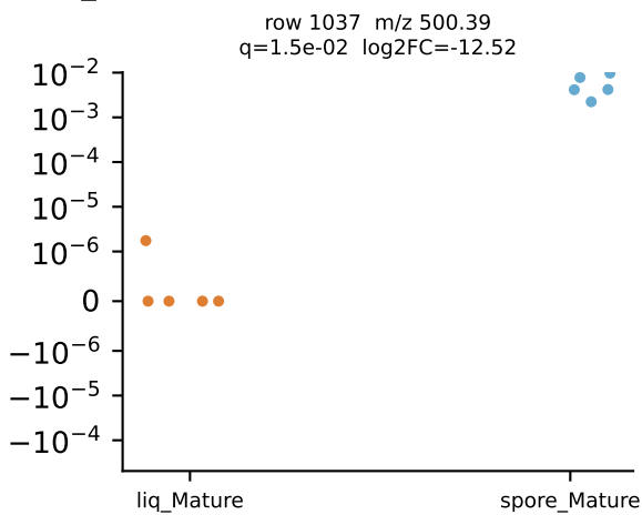
Top 20 differential features: liq_Mature vs spore_Mature (TSS proportion, symlog y)
