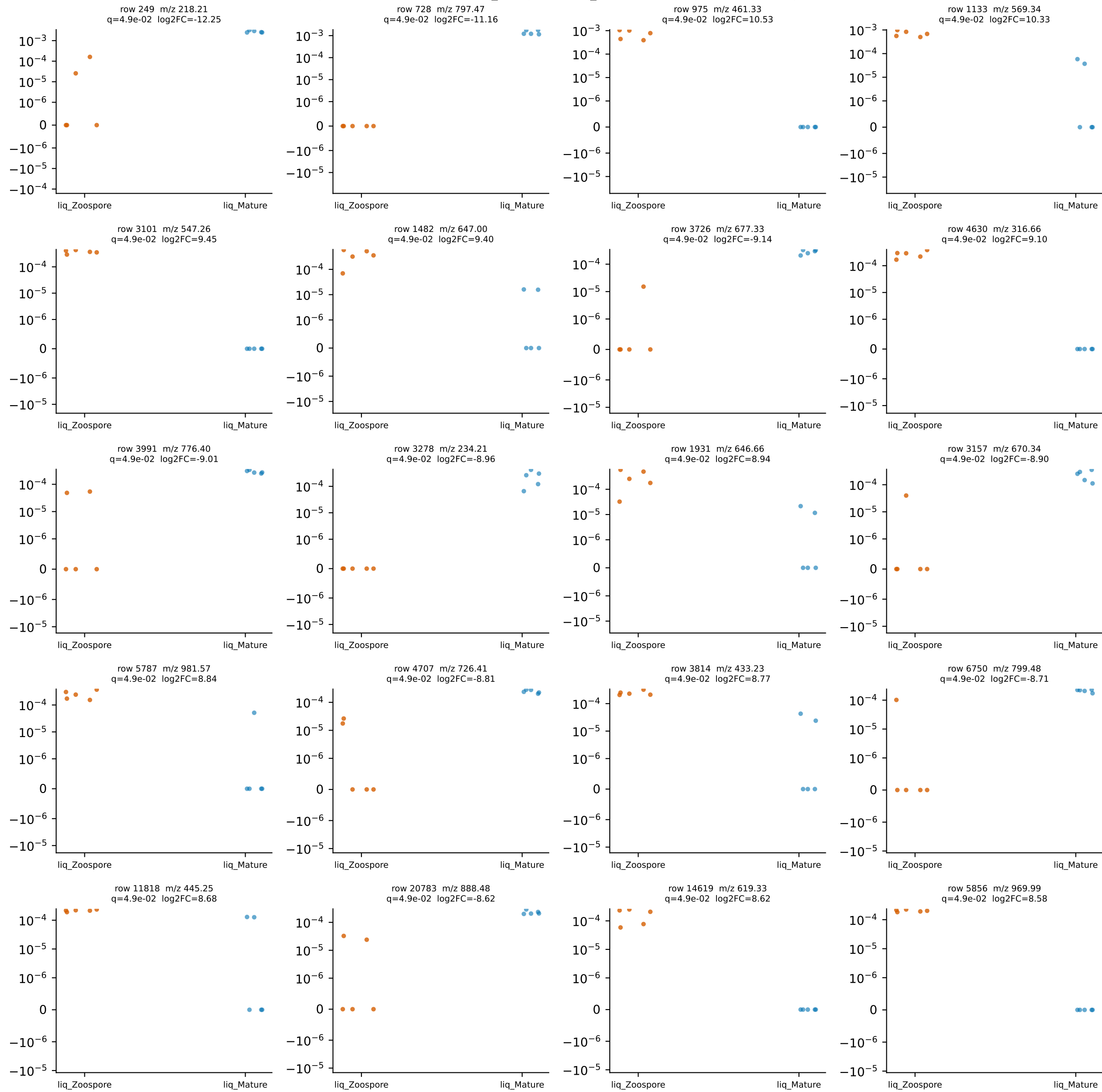
Top 20 differential features: liq_Zoospore vs liq_Mature (TSS proportion, symlog y)
