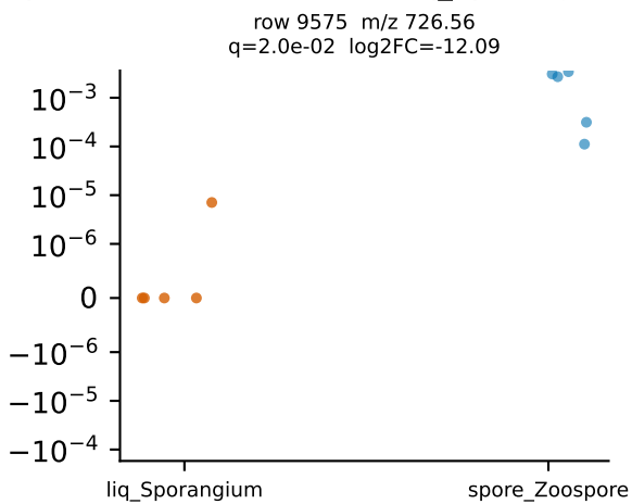
Top 20 differential features: liq_Sporangium vs spore_Zoospore (TSS proportion, symlog y)
