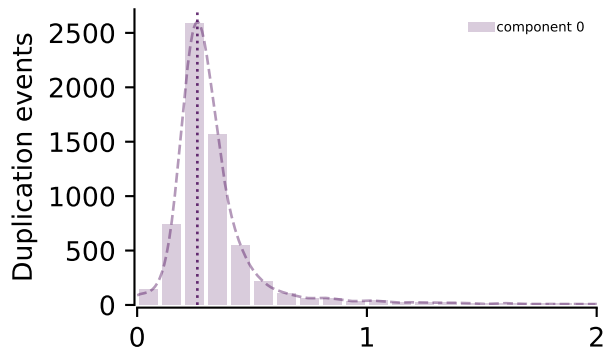
Ks_gmm_1components_prediction.tsv
