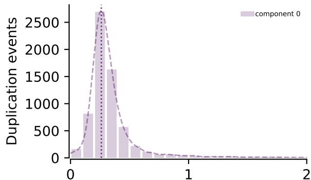
Ks_gmm_1components_prediction.tsv
