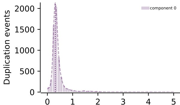
Ks_gmm_1components_prediction.tsv
