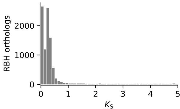
Orthogroups.sp.tsv
