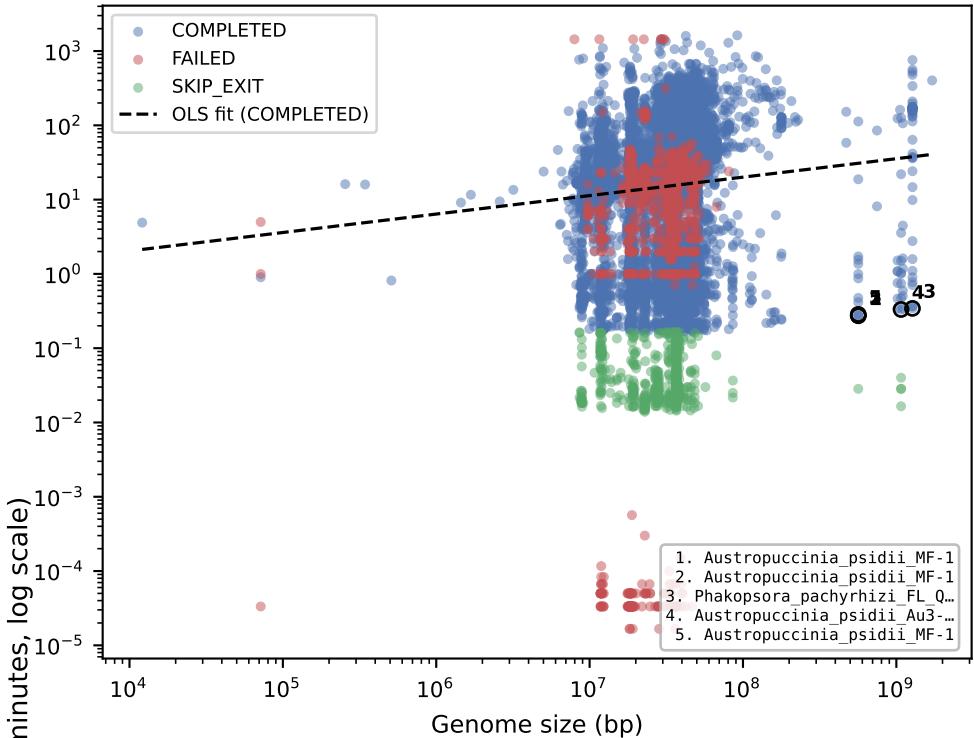
FUNANNOTATE_PREDICT_SIB (n=1061)
