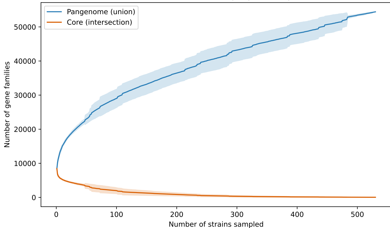
Accumulation curve (Heaps' \gamma=0.33 , open)
