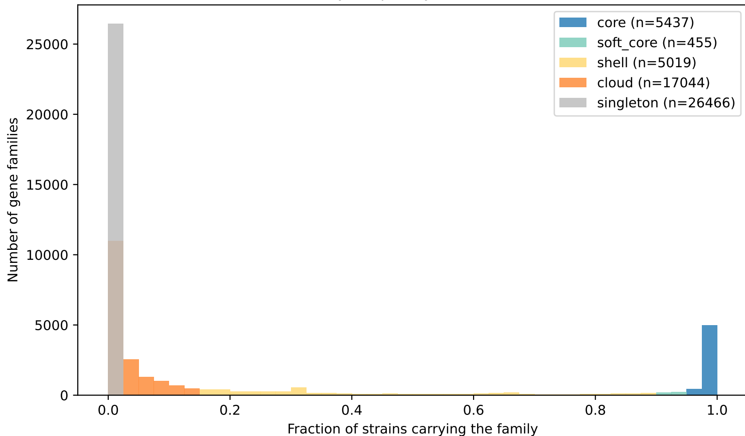
Family-frequency distribution
