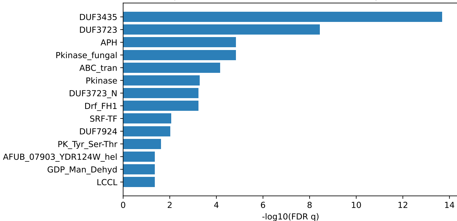
Top 14 enriched Pfam domains in accessory islands
