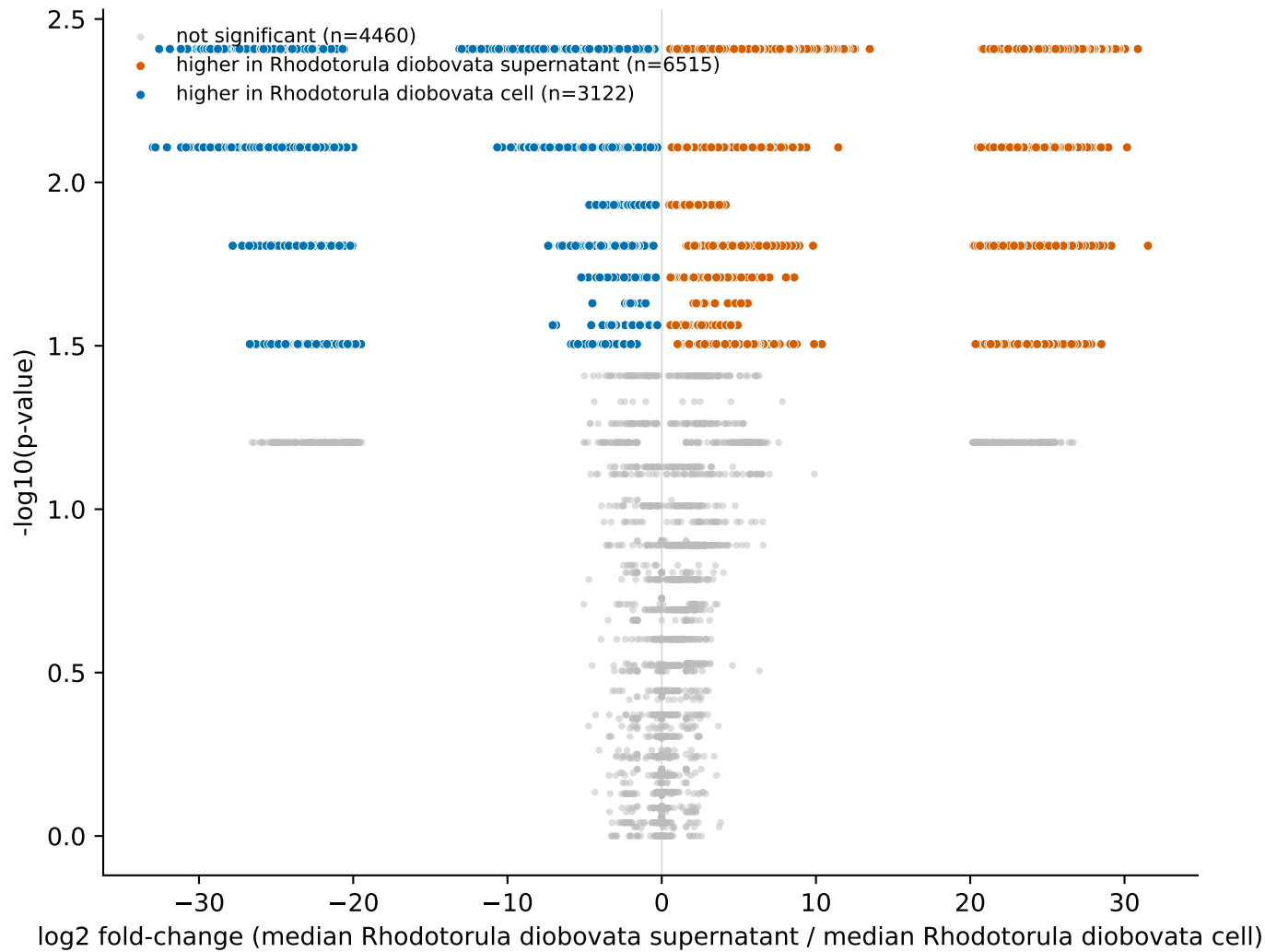
Differential MS2 features: Rhodotorula diobovata supernatant vs Rhodotorula diobovata cell (FDR < 5% colored)
