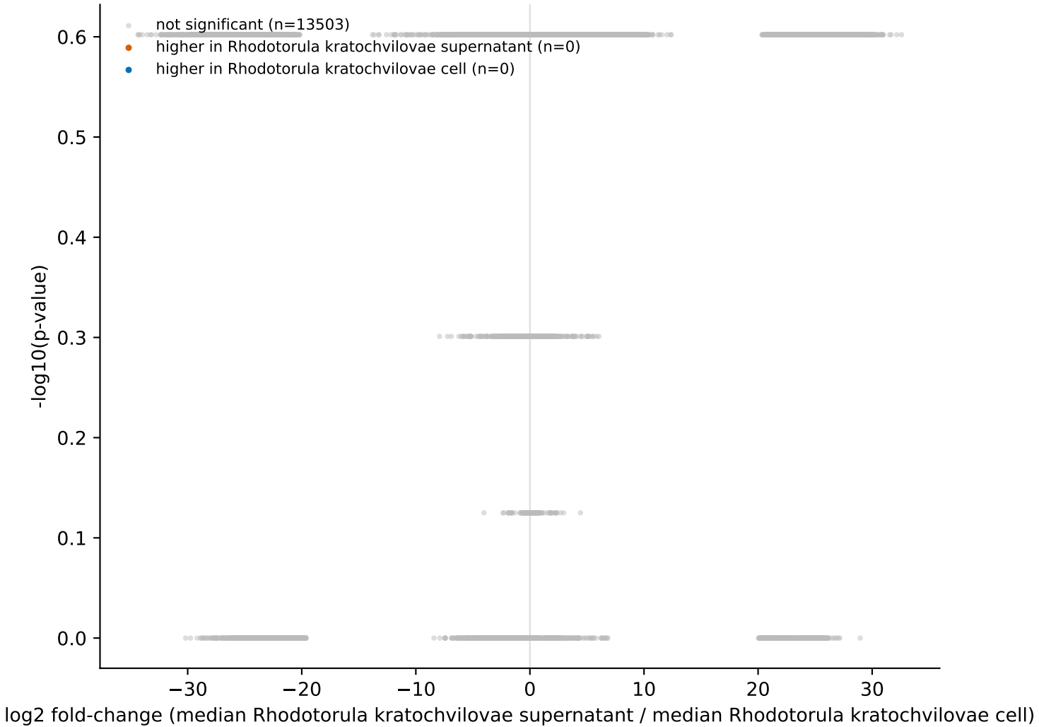
Differential MS2 features: Rhodotorula kratochvilovae supernatant vs Rhodotorula kratochvilovae cell (FDR < 5% colored)
