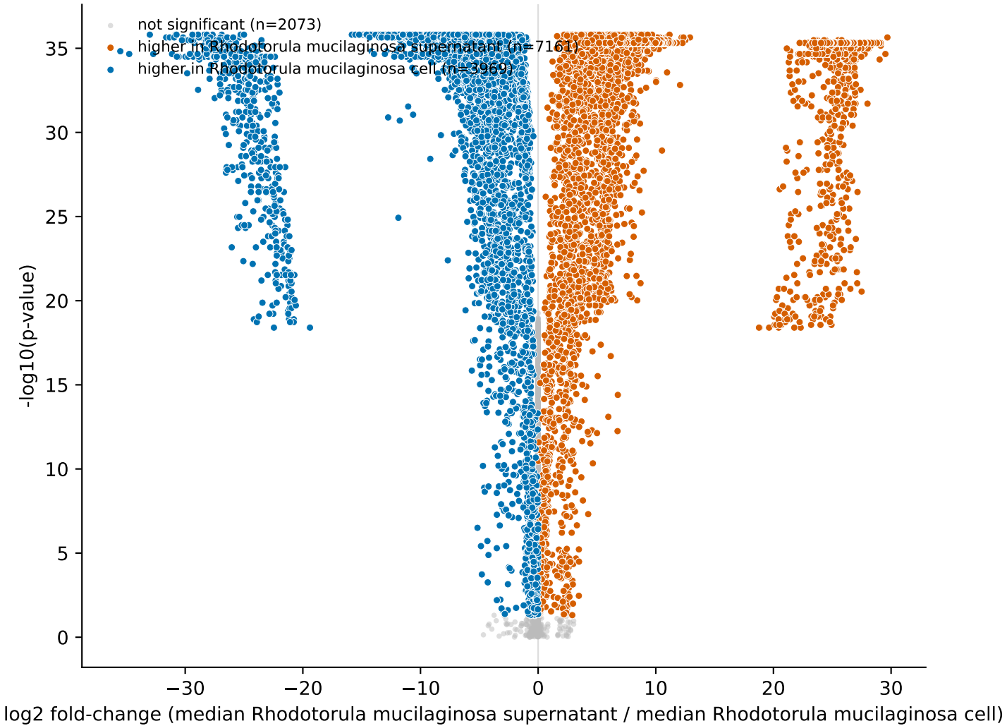
Differential MS2 features: Rhodotorula mucilaginosa supernatant vs Rhodotorula mucilaginosa cell (FDR < 5% colored)
