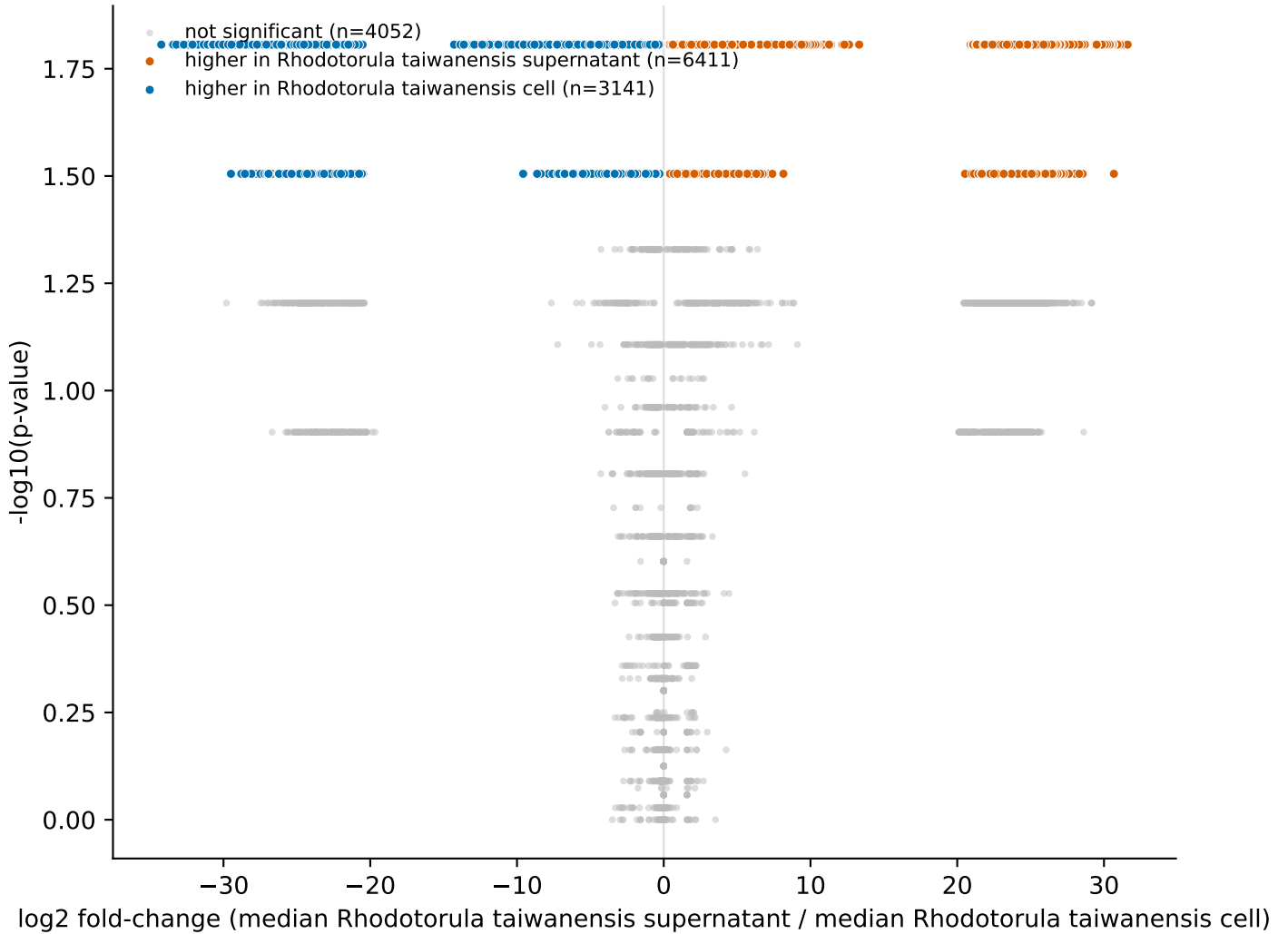
Differential MS2 features: Rhodotorula taiwanensis supernatant vs Rhodotorula taiwanensis cell (FDR < 5% colored)
