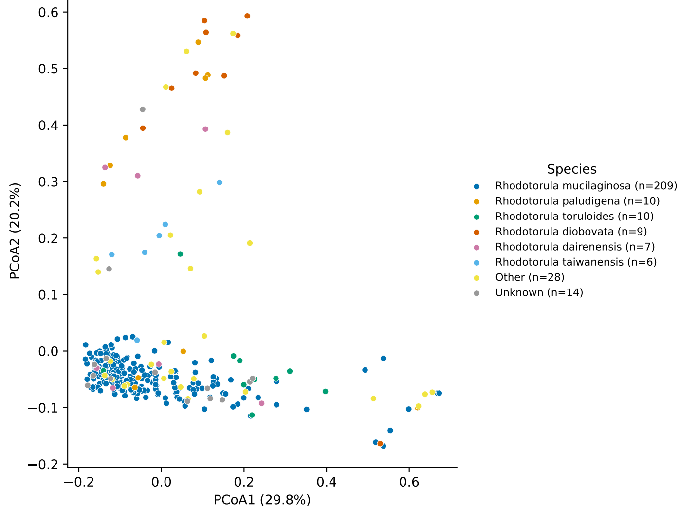
Bray-Curtis PCoA of MS2 features -- cell pellet only
